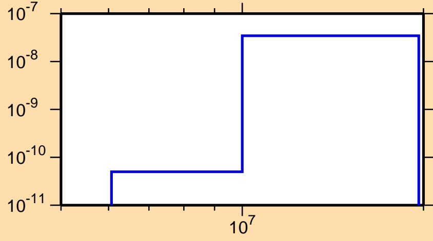
\sigma vs. E for ^{241}\text{Cf}(n,2n\alpha)
