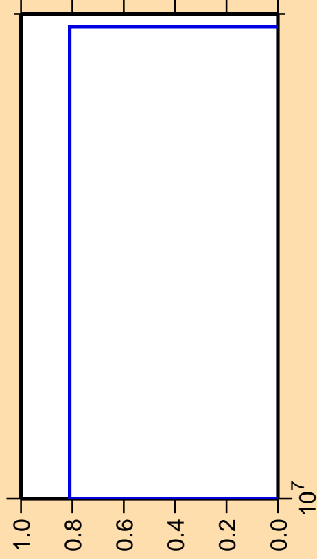
\Delta\sigma/\sigma vs. E for ^{241}\text{Cf} (mt 34)
