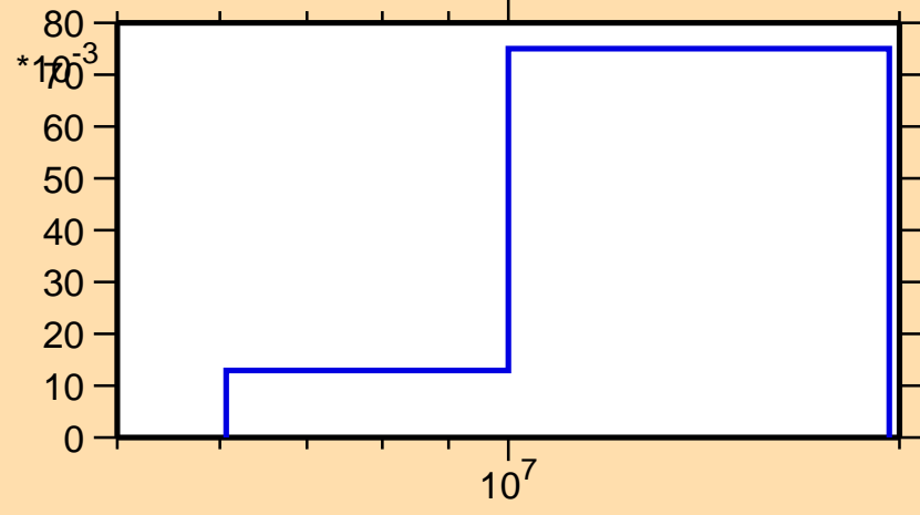
\sigma vs. E for ^{241}\text{Cf}(n,2n)
