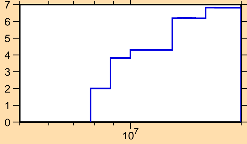
\Delta\sigma/\sigma vs. E for ^{242}\text{Cf}(n,\text{nonel.})
