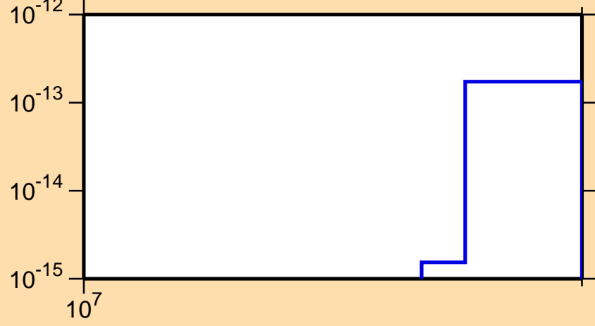
\sigma vs. E for ^{242}\text{Cf} (mt 34)
