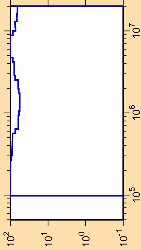
\Delta\sigma/\sigma vs. E for ^{242}\text{Cf}(n,\text{inel.})
