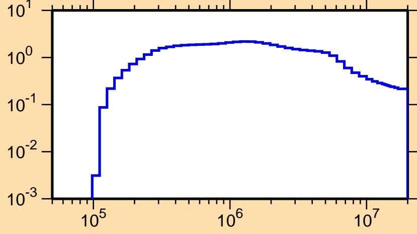
\sigma vs. E for ^{242}\text{Cf}(n,\text{inel.})
