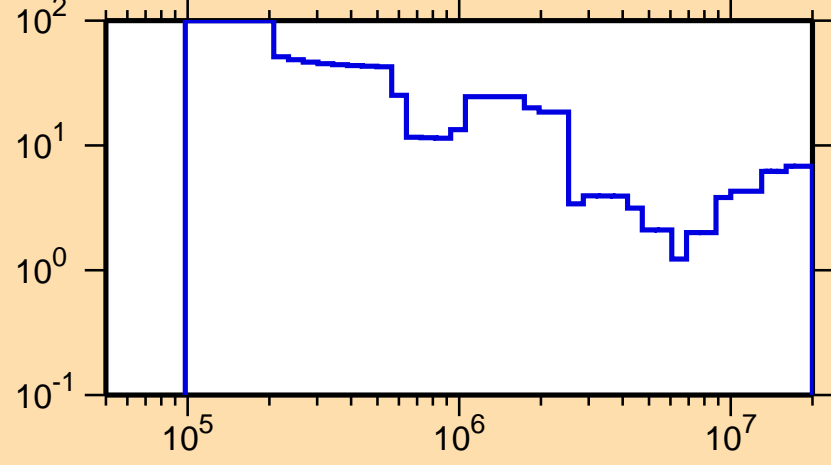
\Delta\sigma/\sigma vs. E for ^{242}\text{Cf}(n,\text{nonel.})
