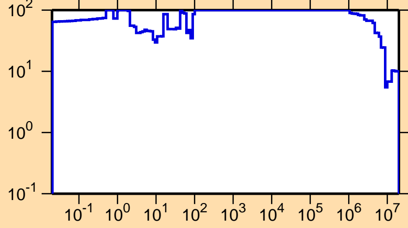
\Delta\sigma/\sigma vs. E for ^{242}\text{Cf}(n,f)
