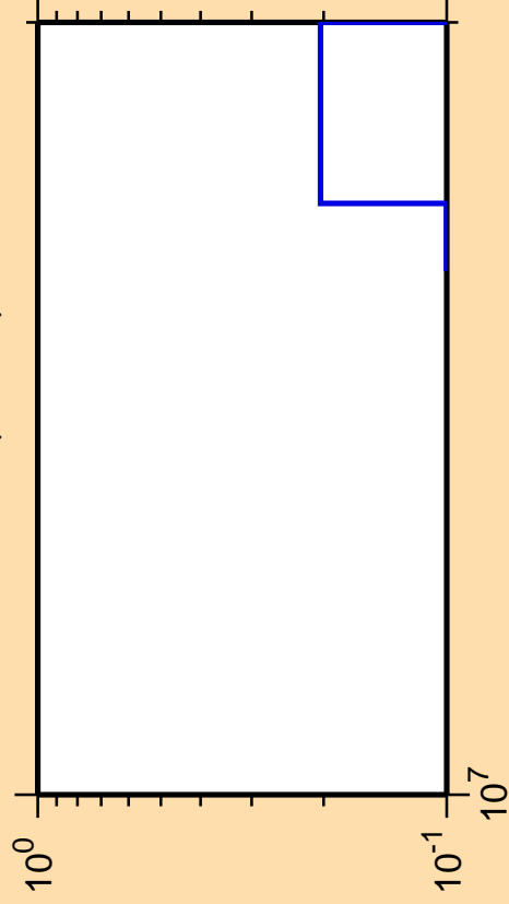
\Delta\sigma/\sigma vs. E for ^{242}\text{Cf} (mt 34)
