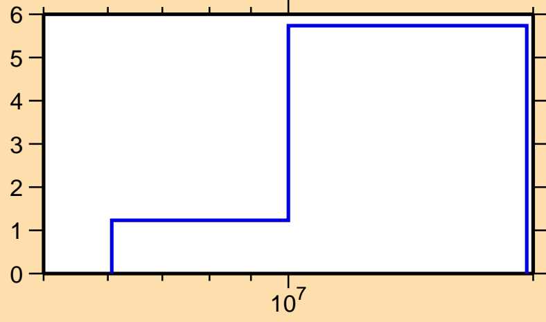
\Delta\sigma/\sigma vs. E for ^{242}\text{Cf}(n,\text{nonel.})
