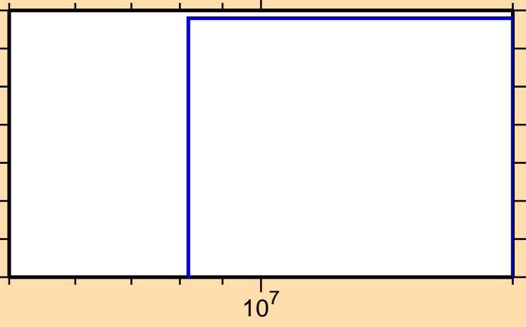
\sigma vs. E for ^{242}\text{Cf}(n,2np)
