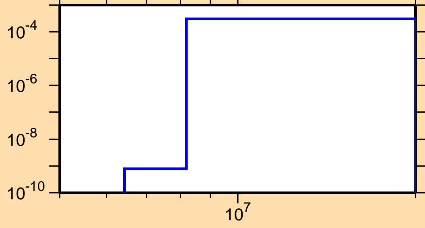
\sigma vs. E for ^{242}\text{Cf}(n,np)
