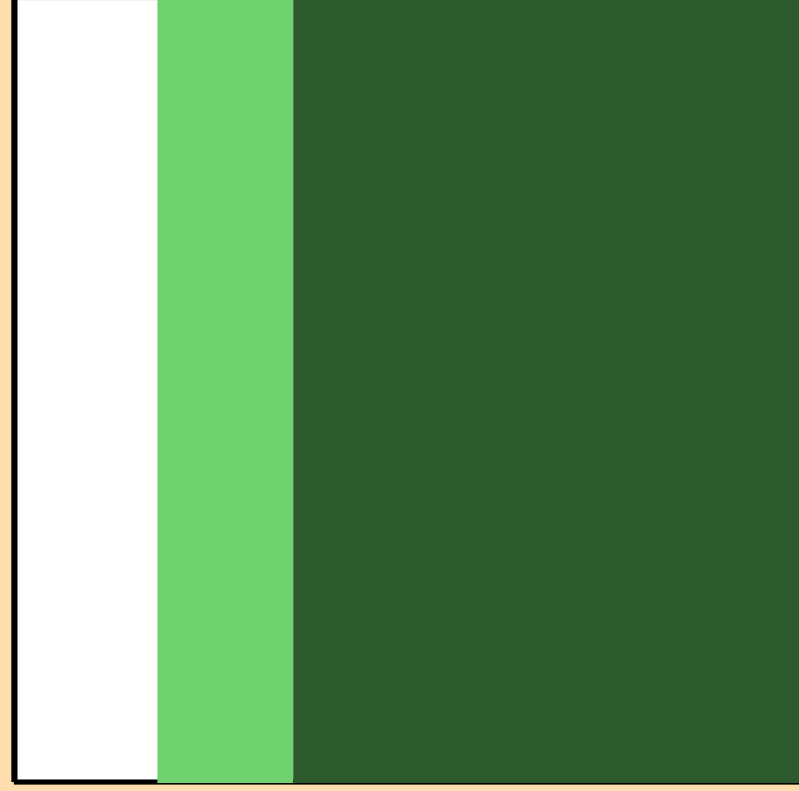
\Delta\sigma/\sigma vs. E for ^{242}\text{Cf}(n,2n)
