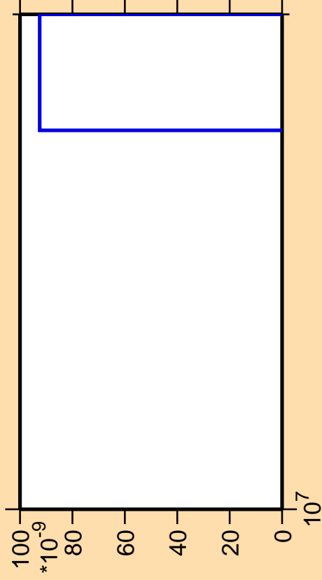
\Delta\sigma/\sigma vs. E for ^{243}\text{Cf} (mt 42)
