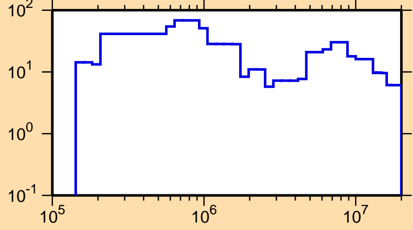
\Delta\sigma/\sigma vs. E for ^{243}\text{Cf}(n,\text{el.})
