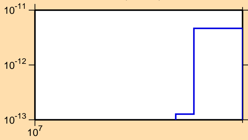
\sigma vs. E for ^{243}\text{Cf} (mt 34)
