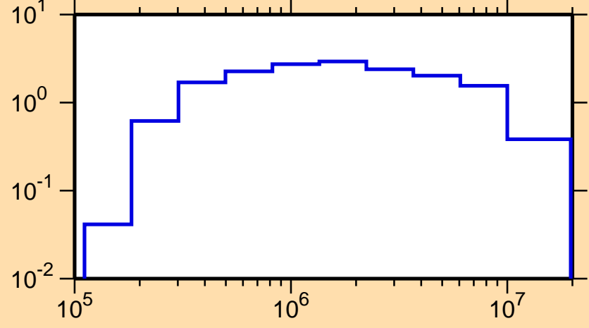
\sigma vs. E for ^{243}\text{Cf}(n,\text{inel.})
