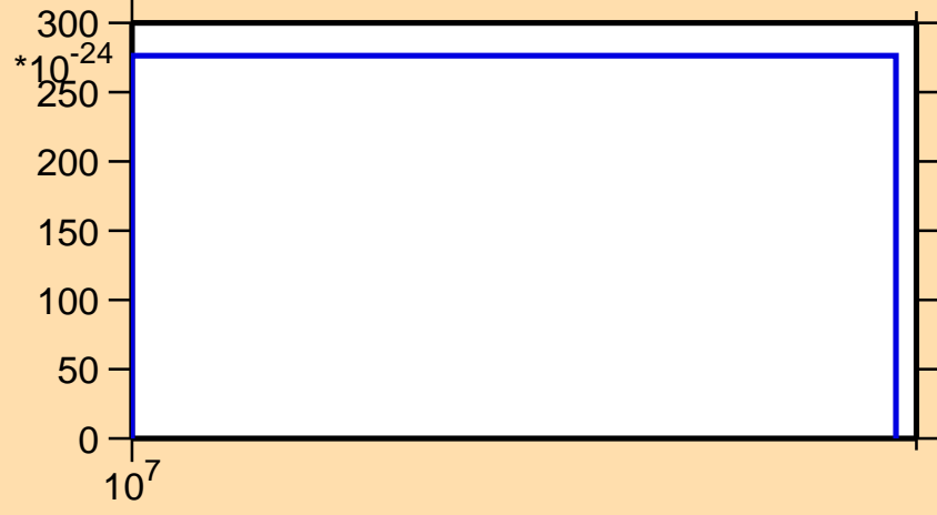
\sigma vs. E for ^{243}\text{Cf} (mt 42)
