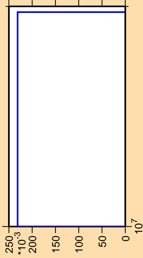
\Delta\sigma/\sigma vs. E for ^{243}\text{Cf} (mt 34)
