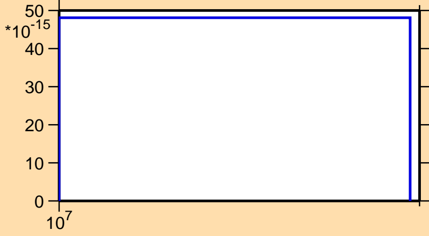
\sigma vs. E for ^{243}\text{Cf} (mt 34)
