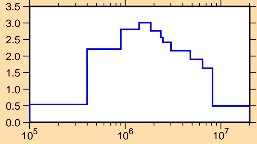
\sigma vs. E for ^{243}\text{Cf}(n,\text{inel.})
