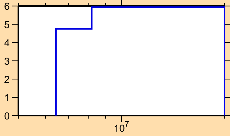
\Delta\sigma/\sigma vs. E for ^{243}\text{Cf}(n,\text{nonel.})
