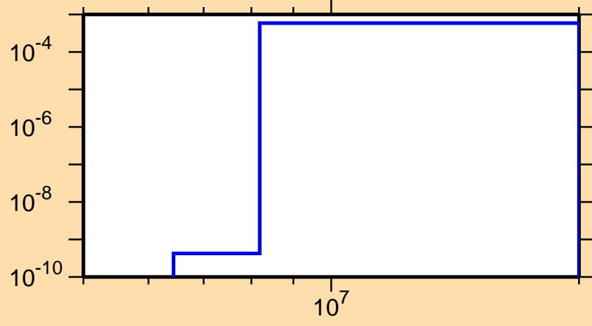
\sigma vs. E for ^{243}\text{Cf}(n,d)
