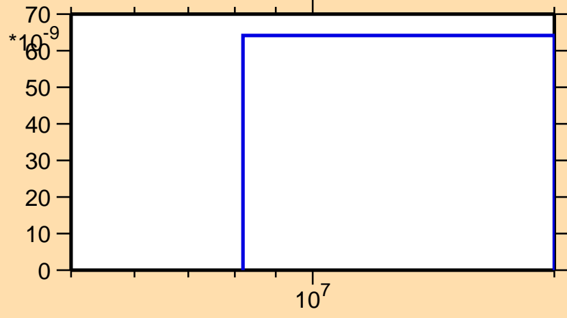
\sigma vs. E for ^{243}\text{Cf}(n,nd)
