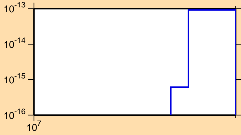
\sigma vs. E for ^{244}\text{Cf} (mt 34)
