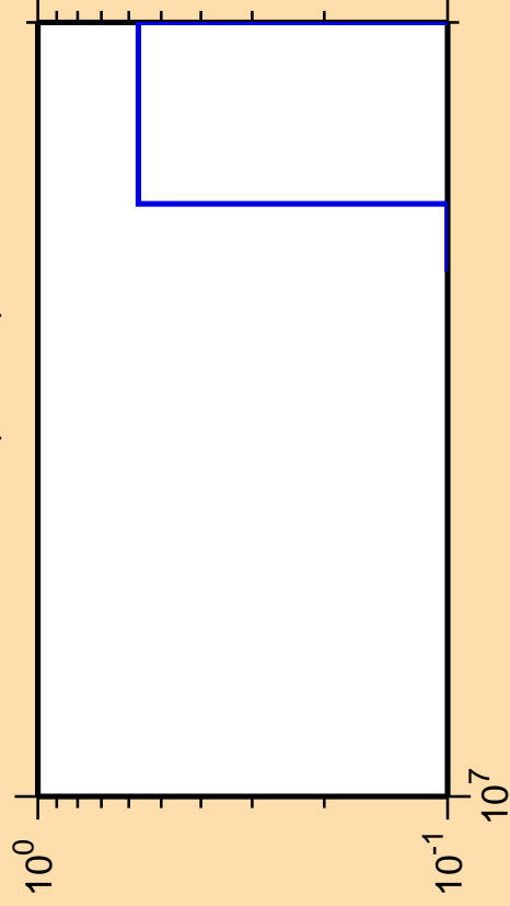
\Delta\sigma/\sigma vs. E for ^{244}\text{Cf} (mt 34)
