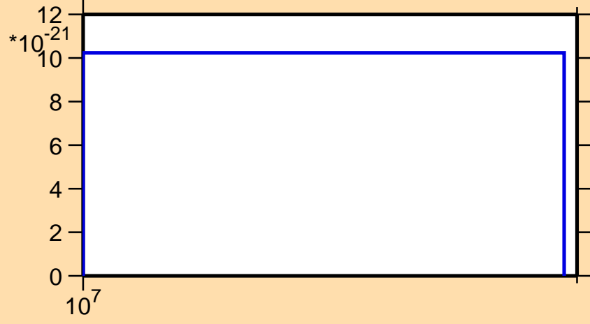
\sigma vs. E for ^{244}\text{Cf} (mt 42)
