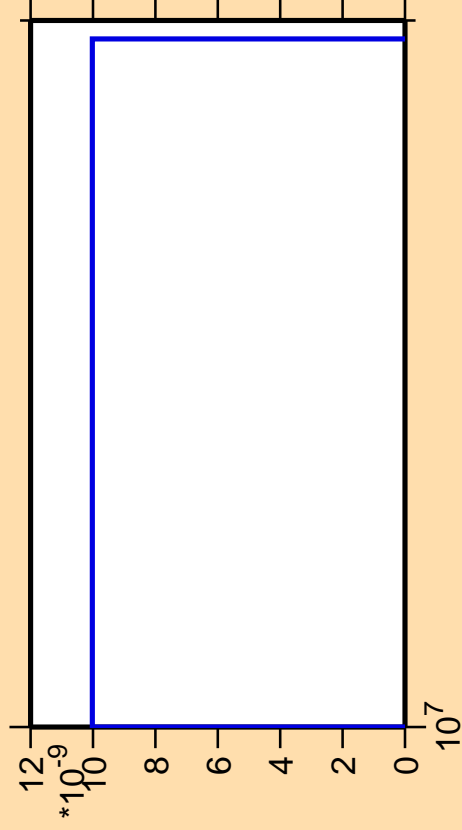
\Delta\sigma/\sigma vs. E for ^{244}\text{Cf} (mt 42)
