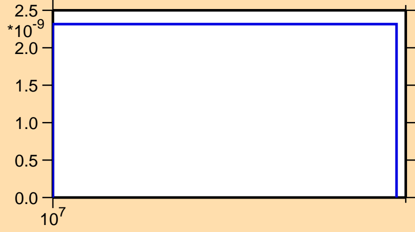
\sigma vs. E for ^{244}\text{Cf}(n,nt)
