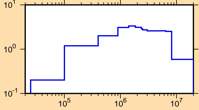
\sigma vs. E for ^{244}\text{Cf}(n,\text{inel.})
