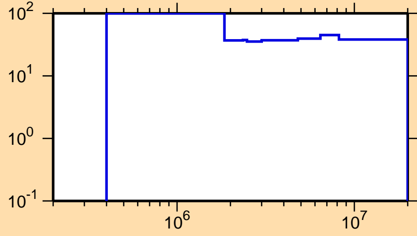
\Delta\sigma/\sigma vs. E for ^{244}\text{Cf}(n,ncont.)
