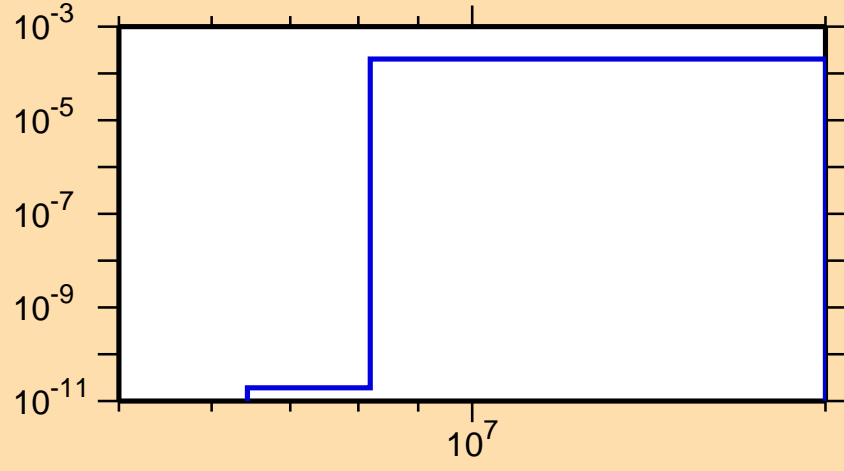
\sigma vs. E for ^{244}\text{Cf}(n,d)
