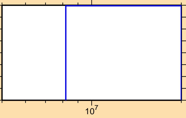
\sigma vs. E for ^{244}\text{Cf}(\text{mt117})
