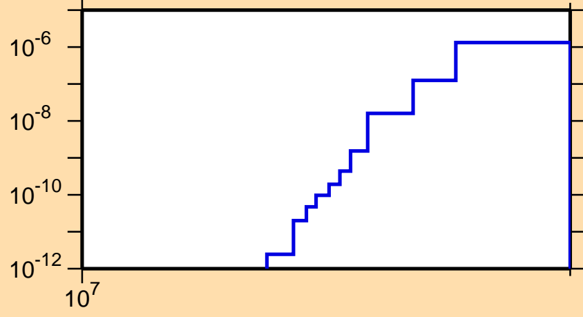
\sigma vs. E for ^{245}\text{Cf}(n,nd)
