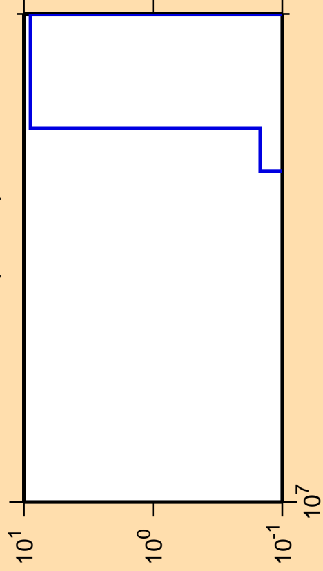
\Delta\sigma/\sigma vs. E for ^{245}\text{Cf} (mt 34)
