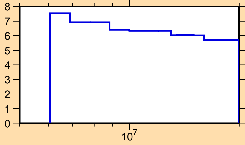
\Delta\sigma/\sigma vs. E for ^{245}\text{Cf}(n,\text{nonel.})
