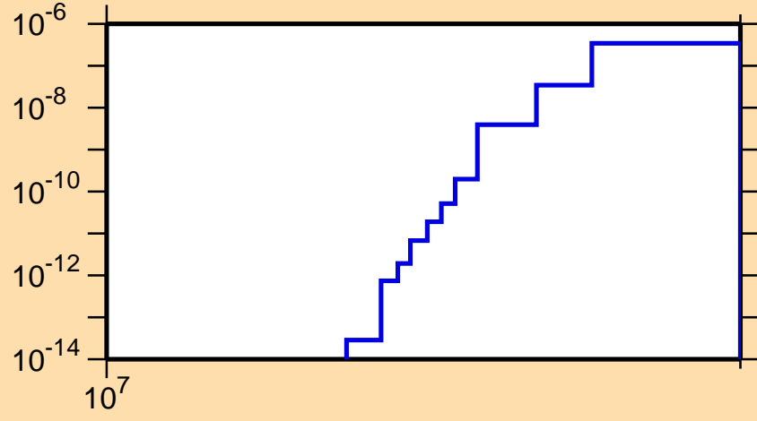
\sigma vs. E for ^{245}\text{Cf}(n,2np)
