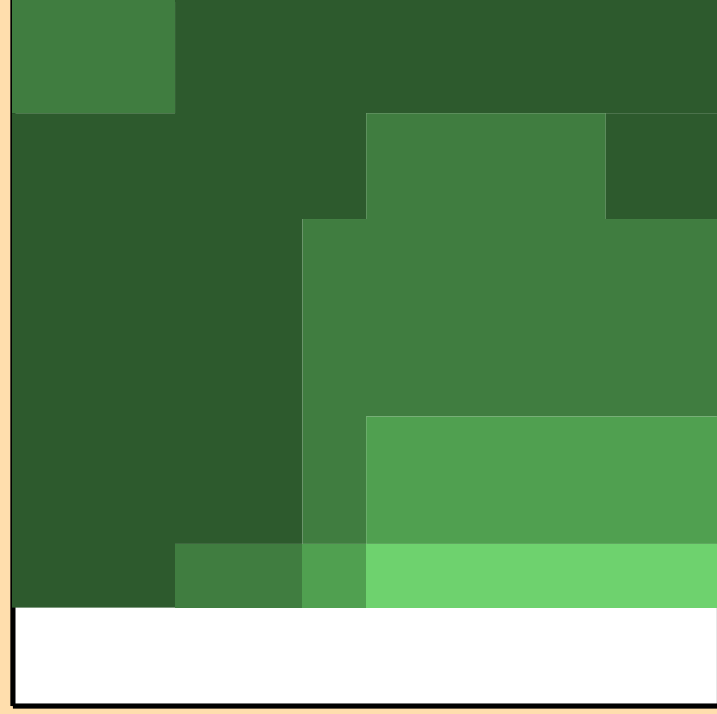
\Delta\sigma/\sigma vs. E for ^{245}\text{Cf}(n,\text{inel.})
