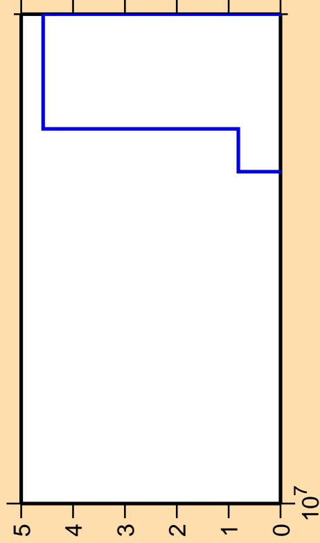
\Delta\sigma/\sigma vs. E for ^{245}\text{Cf}(\text{mt117})
