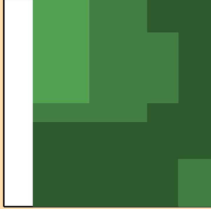
\Delta\sigma/\sigma vs. E for ^{245}\text{Cf}(n,2n)
