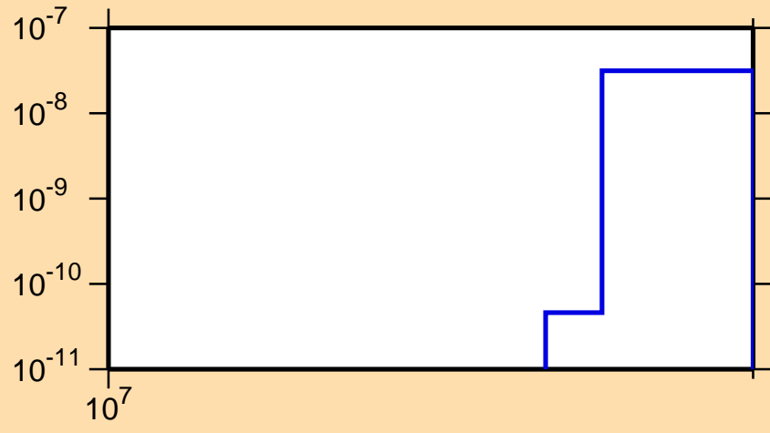
\sigma vs. E for ^{245}\text{Cf}(n,3n\alpha)
