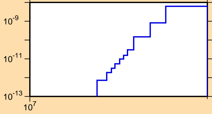
\sigma vs. E for ^{245}\text{Cf}(n,\text{He3})
