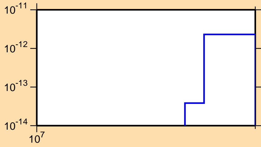
\sigma vs. E for ^{245}\text{Cf} (mt 34)
