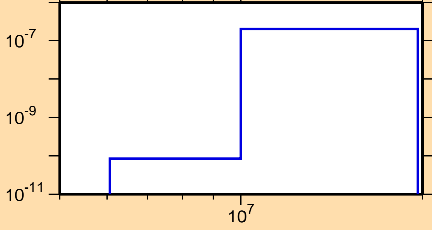
\sigma vs. E for ^{245}\text{Cf}(n,2n\alpha)
