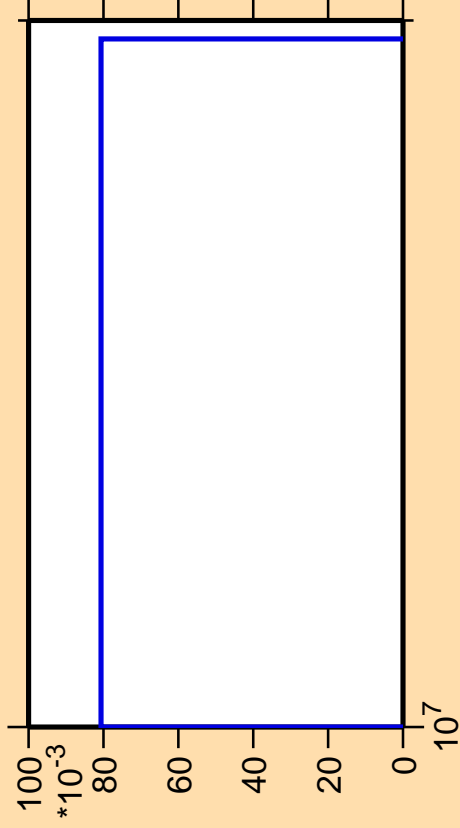
\Delta\sigma/\sigma vs. E for ^{245}\text{Cf} (mt 34)
