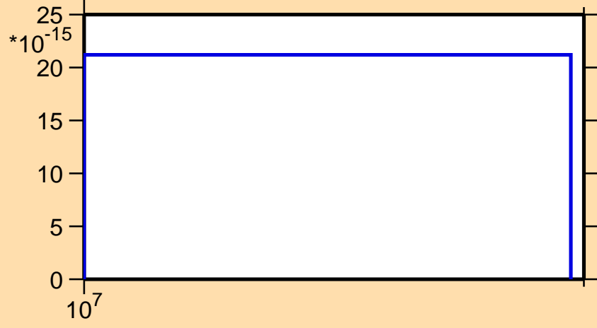
\sigma vs. E for ^{245}\text{Cf} (mt 34)
