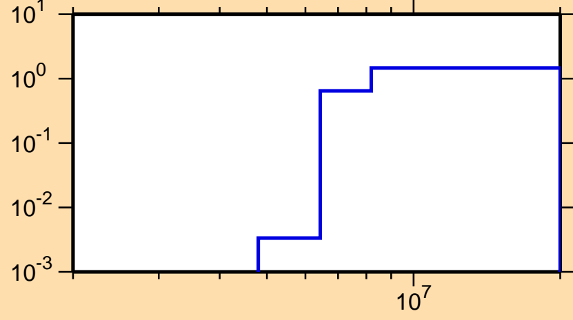
\sigma vs. E for ^{245}\text{Cf}(n,2n)
