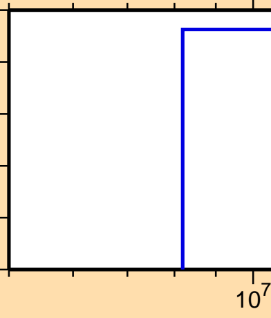
\sigma vs. E for ^{245}\text{Cf}(n,2np)
