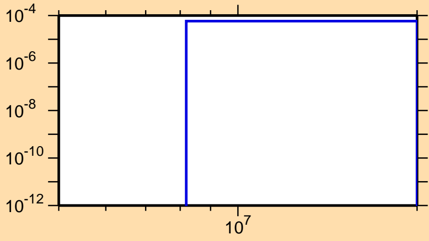
\sigma vs. E for ^{245}\text{Cf}(n,t)
