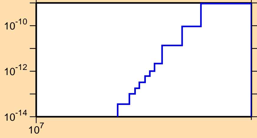
\sigma vs. E for ^{246}\text{Cf}(n,\text{He3})
