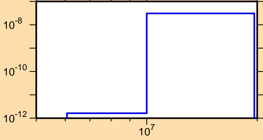
\sigma vs. E for ^{246}\text{Cf}(n,2n\alpha)
