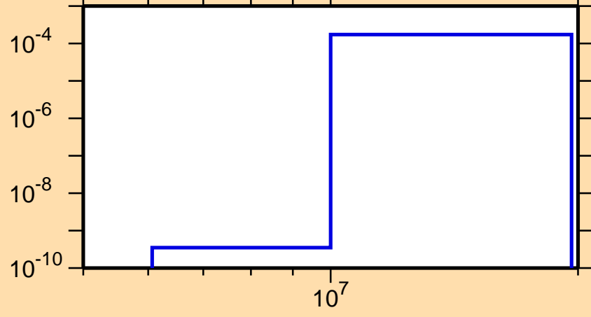
\sigma vs. E for ^{246}\text{Cf}(n,d)
