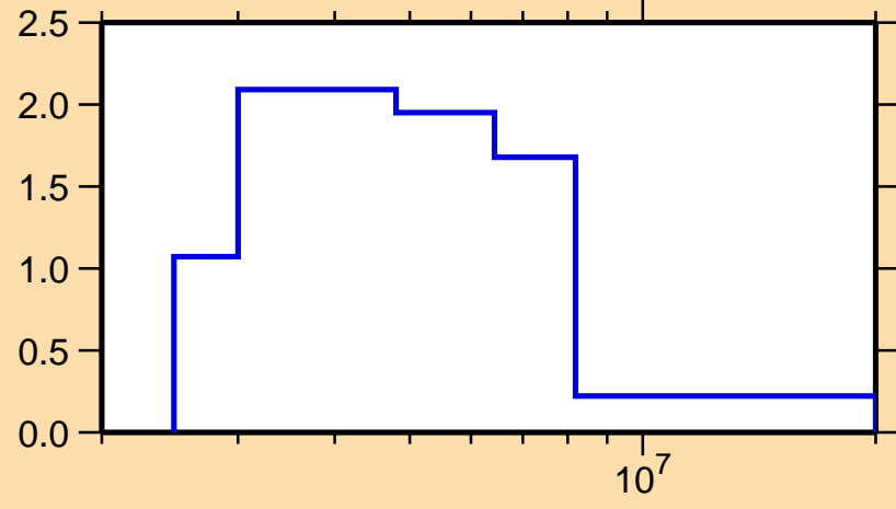
\sigma vs. E for ^{246}\text{Cf}(n,n\text{cont.})
