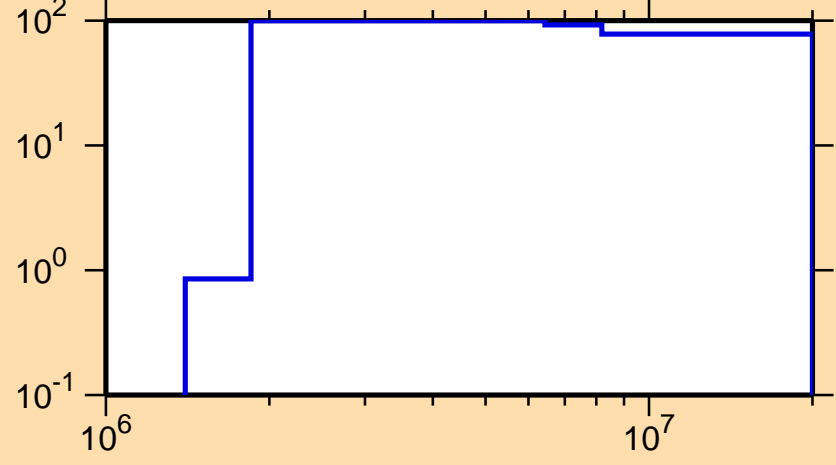
\Delta\sigma/\sigma vs. E for ^{246}\text{Cf}(n,p)
