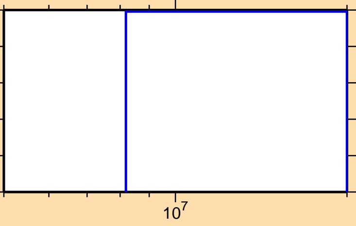
\sigma vs. E for ^{246}\text{Cf}(n,2n\alpha)
