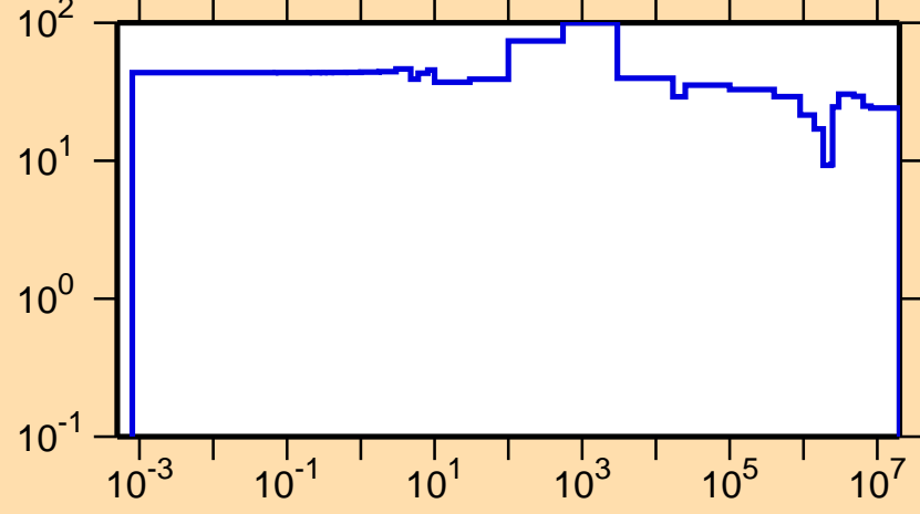
\Delta\sigma/\sigma vs. E for ^{246}\text{Cf}(n,\text{el.})
