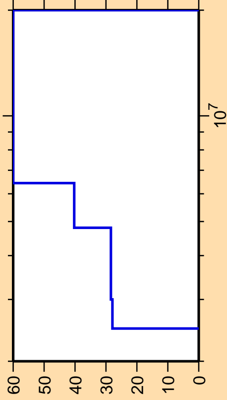
\Delta\sigma/\sigma vs. E for ^{246}\text{Cf}(n, ncont.)
