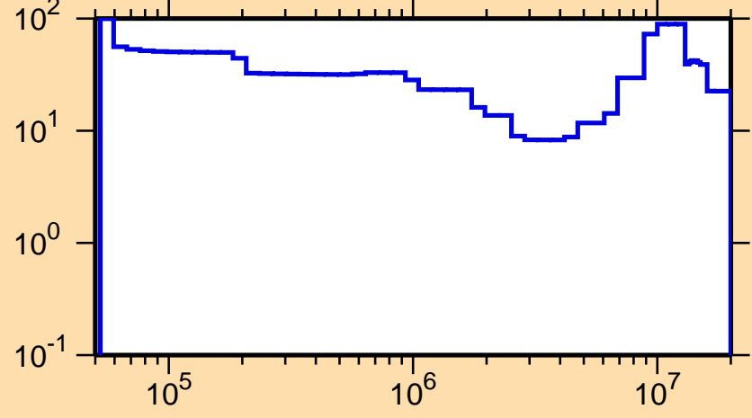
\Delta\sigma/\sigma vs. E for ^{247}\text{Cf}(n,inel.)
