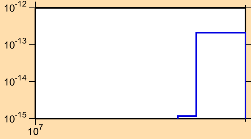
\sigma vs. E for ^{247}\text{Cf} (mt 34)
