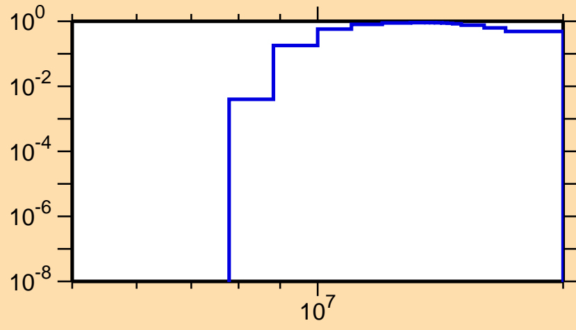
\sigma vs. E for ^{247}\text{Cf}(n,2n\alpha)
