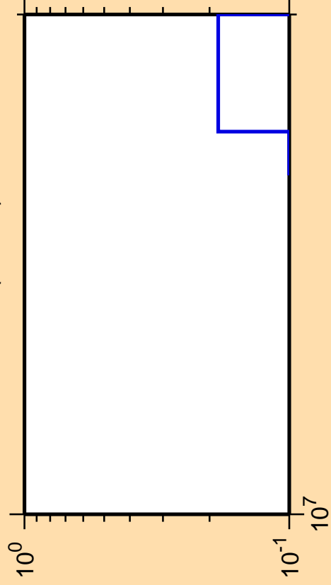
\Delta\sigma/\sigma vs. E for ^{247}\text{Cf} (mt 34)
