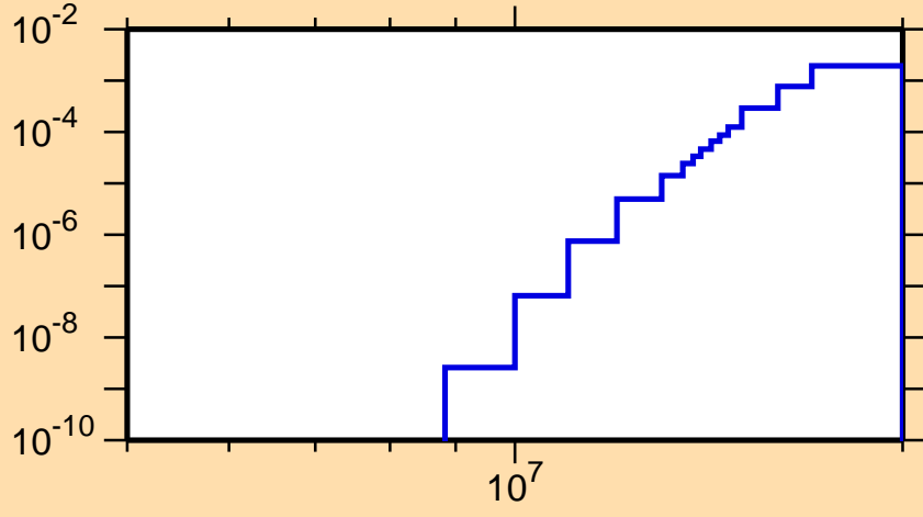
\sigma vs. E for ^{247}\text{Cf}(n,np)
