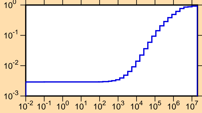
\mu vs. E for ^{247}\text{Cf}(\text{mt251})
