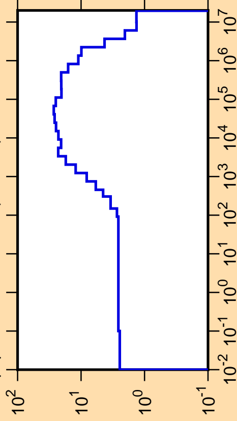
\Delta\mu/\mu vs. E for ^{247}\text{Cf}(\text{mt251})
