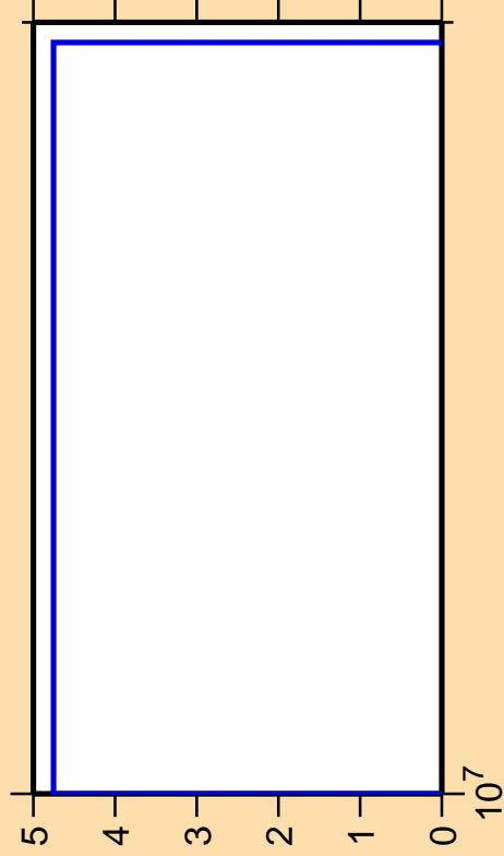
\Delta\sigma/\sigma vs. E for ^{247}\text{Cf}(n,3n\alpha)
