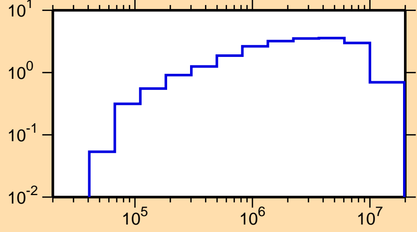
\sigma vs. E for ^{247}\text{Cf}(n,\text{inel.})
