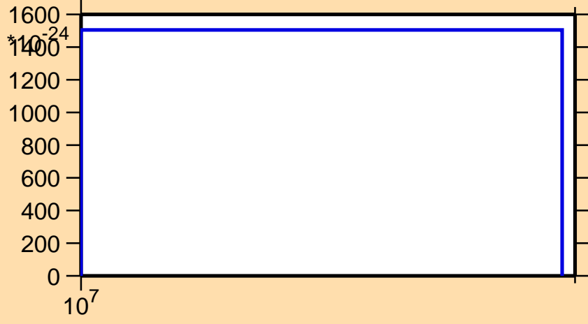
\sigma vs. E for ^{247}\text{Cf} (mt 42)
