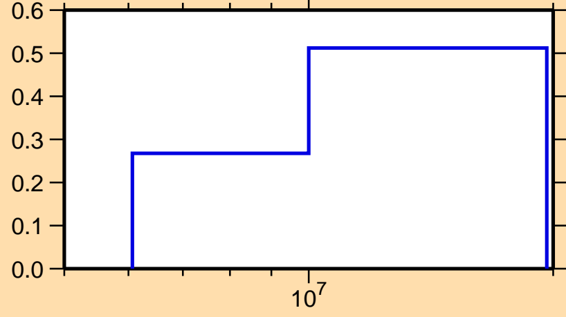
\sigma vs. E for ^{247}\text{Cf}(n,2n)
