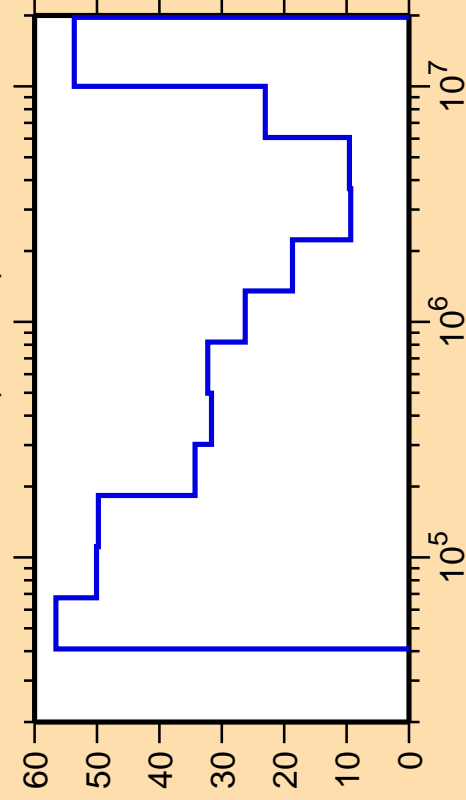
\Delta\sigma/\sigma vs. E for ^{247}\text{Cf}(n,\text{inel.})
