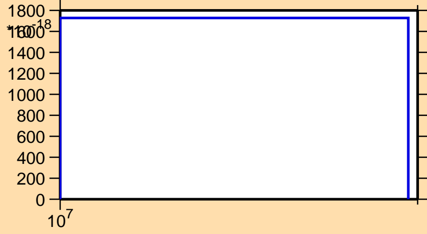
\sigma vs. E for ^{247}\text{Cf}(\text{mt } 34)
