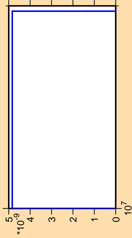
\Delta\sigma/\sigma vs. E for ^{247}\text{Cf} (mt 42)
