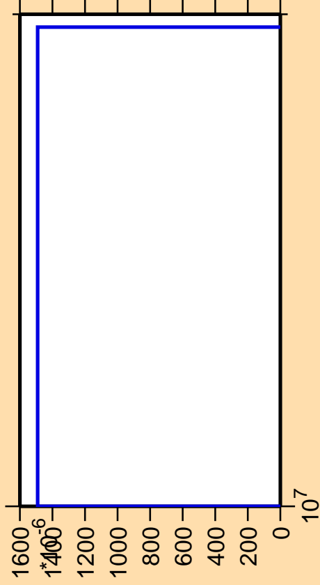
\Delta\sigma/\sigma vs. E for ^{247}\text{Cf}(\text{mt } 34)
