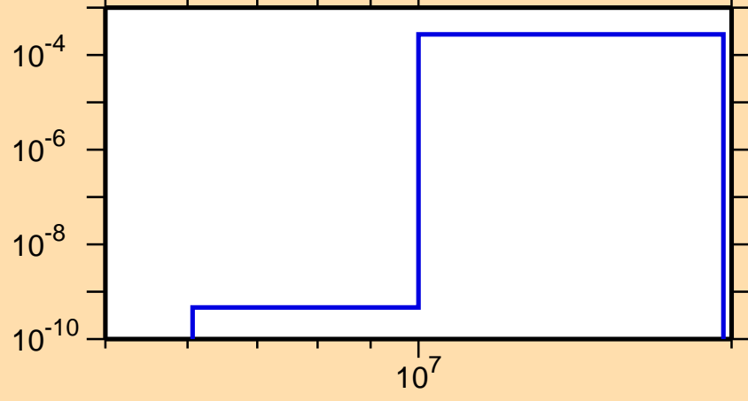
\sigma vs. E for ^{247}\text{Cf}(n,d)
