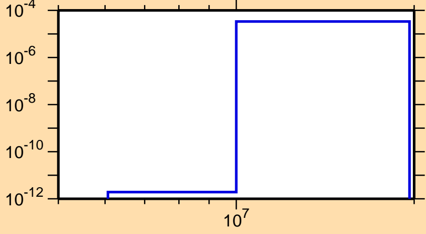
\sigma vs. E for ^{248}\text{Cf}(n,t)
