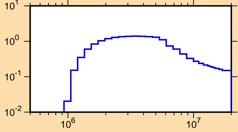
\sigma vs. E for ^{249}\text{Cf}(n,n\text{cont.})
