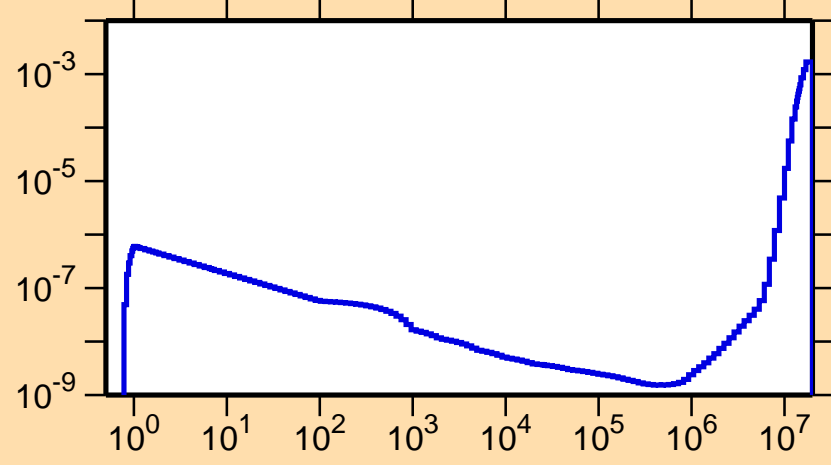
\sigma vs. E for ^{249}\text{Cf}(n,\alpha)
