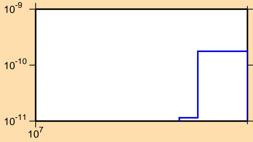
\sigma vs. E for ^{249}\text{Cf}(n,\text{He}3)
