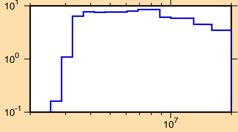
\Delta\sigma/\sigma vs. E for ^{249}\text{Cf}(n,p)
