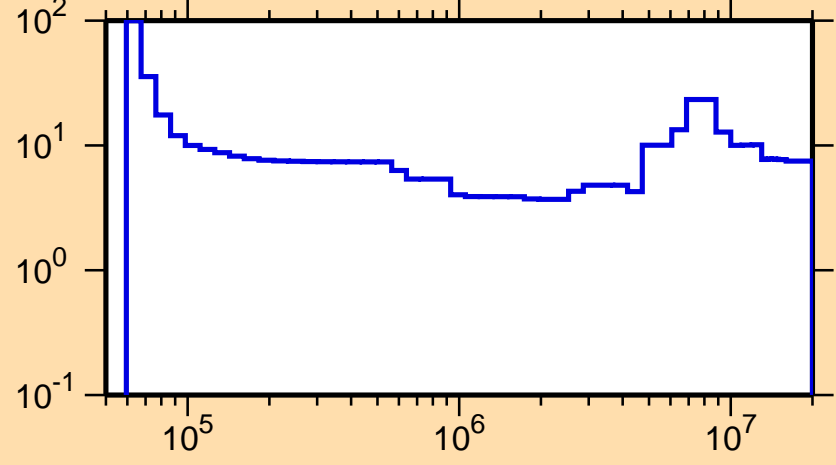
\Delta\sigma/\sigma vs. E for ^{249}\text{Cf}(n,\text{inel.})
