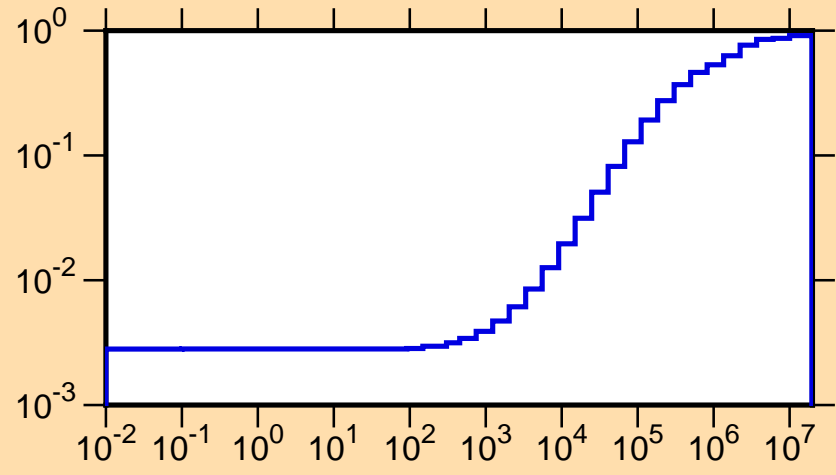
\mu vs. E for ^{249}\text{Cf}(\text{mt251})
