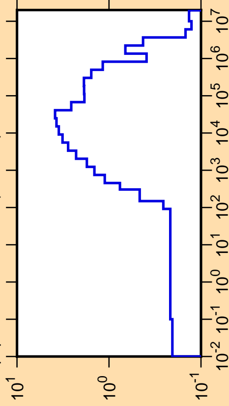
\Delta\mu/\mu vs. E for ^{249}\text{Cf}(\text{mt251})
