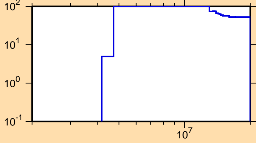
\Delta\sigma/\sigma vs. E for ^{250}\text{Cf}(n,p)
