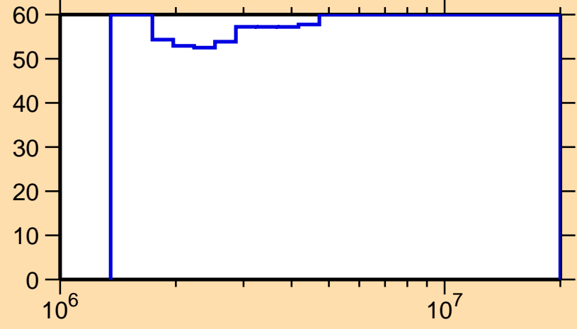
\Delta\sigma/\sigma vs. E for ^{250}\text{Cf}(n,ncont.)
