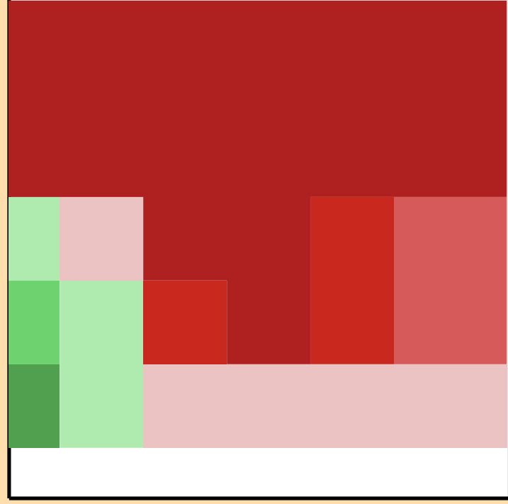
\Delta\sigma/\sigma vs. E for ^{250}\text{Cf}(n, n_1)
