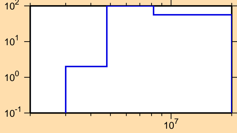
\Delta\sigma/\sigma vs. E for ^{250}\text{Cf}(n,p)
