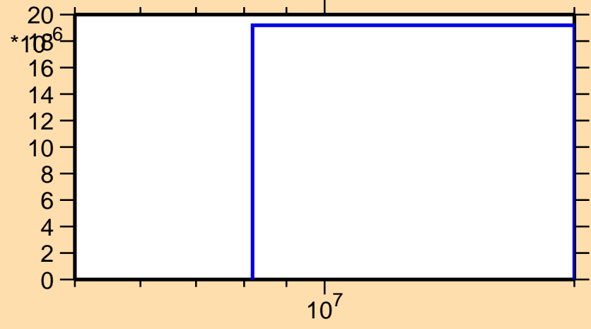
\sigma vs. E for ^{250}\text{Cf}(n,t)
