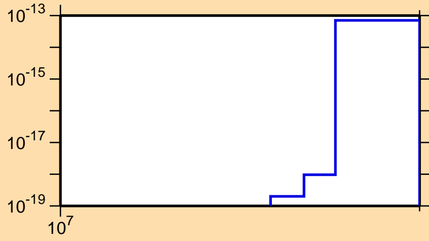
\sigma vs. E for ^{251}\text{Cf} (mt 11)
