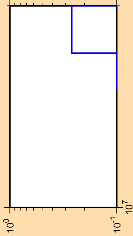
\Delta\sigma/\sigma vs. E for ^{251}\text{Cf} (mt 11)
