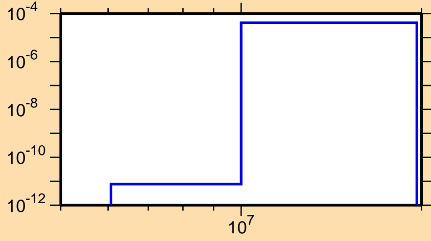
\sigma vs. E for ^{251}\text{Cf}(n,t)
