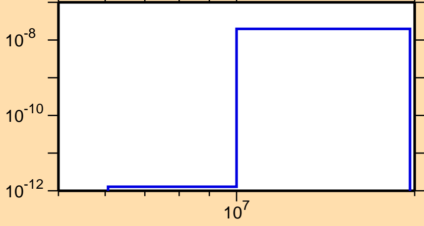
\sigma vs. E for ^{251}\text{Cf}(n,2n\alpha)
