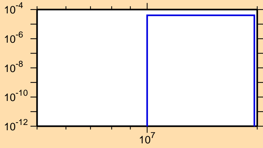
\sigma vs. E for ^{251}\text{Cf}(n,np)
