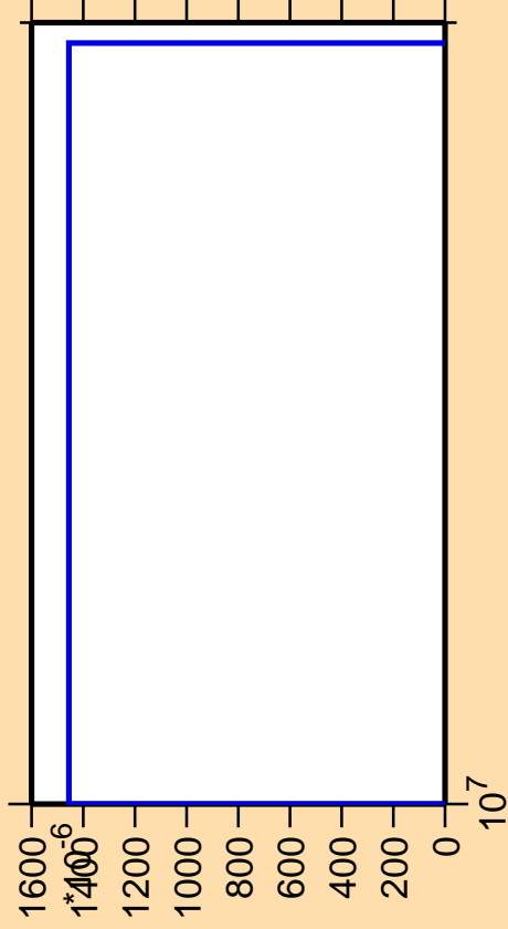
\Delta\sigma/\sigma vs. E for ^{251}\text{Cf}(\text{mt 11})
