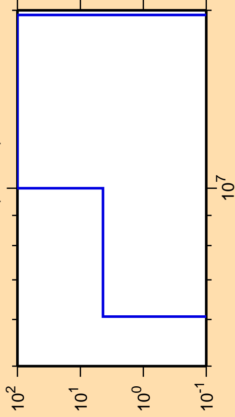
\Delta\sigma/\sigma vs. E for ^{251}\text{Cf}(n,2n\alpha)
