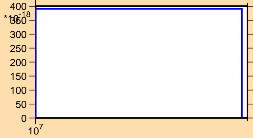
\sigma vs. E for ^{251}\text{Cf}(\text{mt 11})
