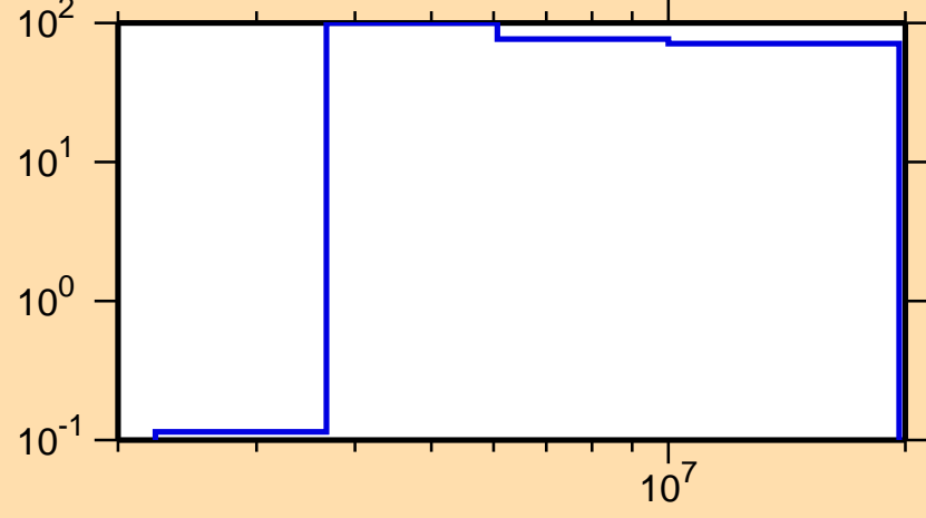
\Delta\sigma/\sigma vs. E for ^{251}\text{Cf}(n,p)
