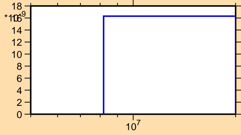
\sigma vs. E for ^{251}\text{Cf}(n,2n\alpha)
