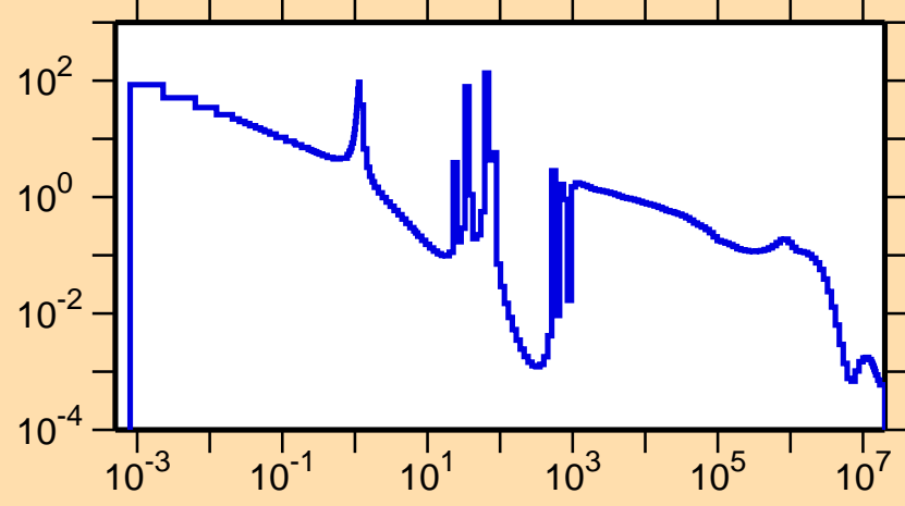
\sigma vs. E for ^{252}\text{Cf}(n,\gamma)
