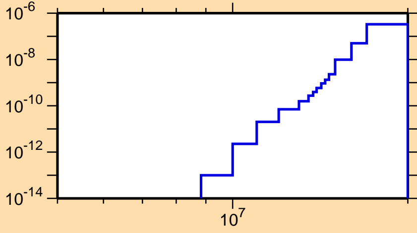
\sigma vs. E for ^{252}\text{Cf}(n,2n\alpha)
