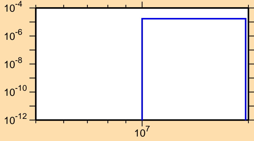
\sigma vs. E for ^{252}\text{Cf}(n,np)
