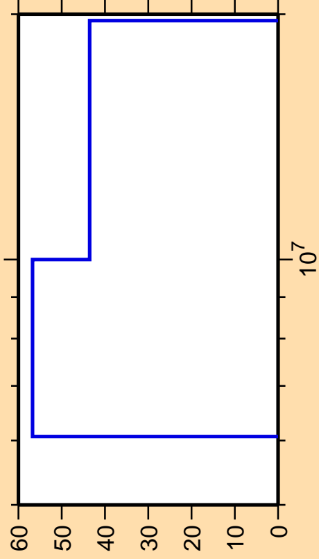
\Delta\sigma/\sigma vs. E for ^{252}\text{Cf}(n,f)
