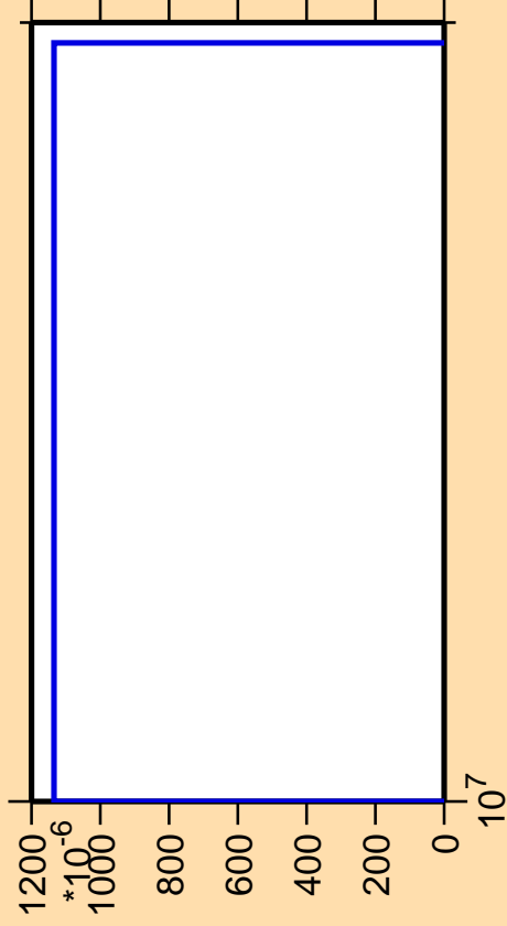
\Delta\sigma/\sigma vs. E for ^{252}\text{Cf} (mt 11)
