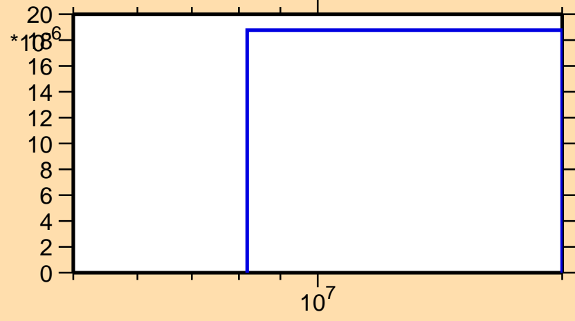
\sigma vs. E for ^{252}\text{Cf}(n,t)
