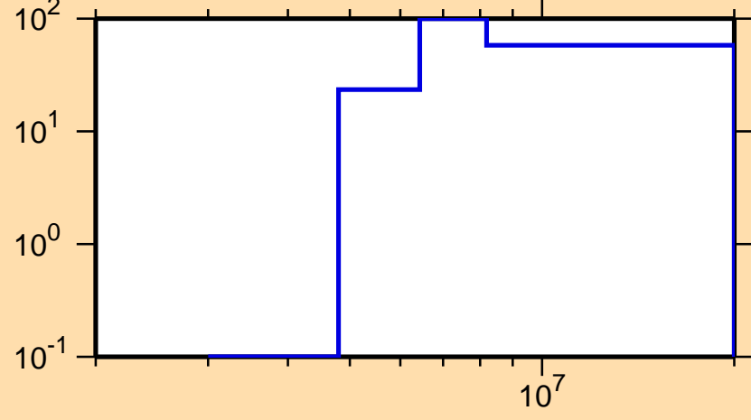
\Delta\sigma/\sigma vs. E for ^{252}\text{Cf}(n,p)
