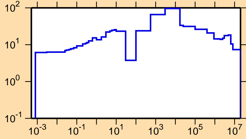
\Delta\sigma/\sigma vs. E for ^{252}\text{Cf}(n,tot.)
