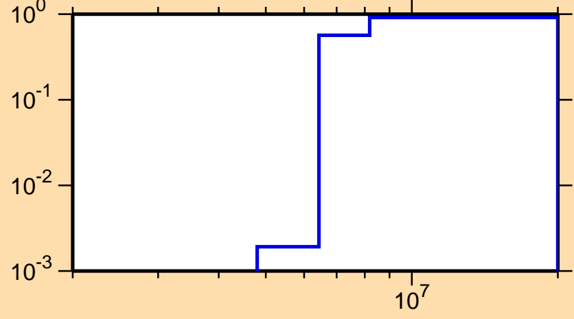
\sigma vs. E for ^{252}\text{Cf}(n,2n)
