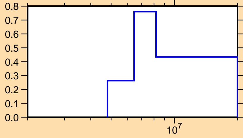
\sigma vs. E for ^{253}\text{Cf}(n,2n)
