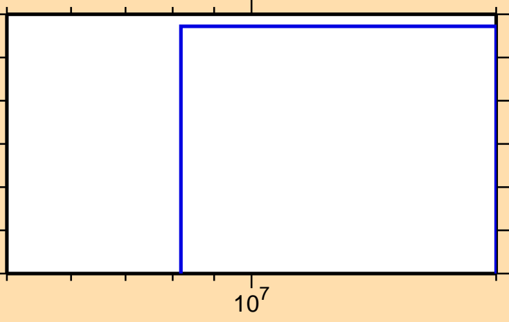
\sigma vs. E for ^{253}\text{Cf}(n,nt)
