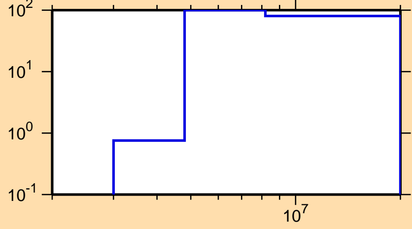
\Delta\sigma/\sigma vs. E for ^{253}\text{Cf}(n,p)
