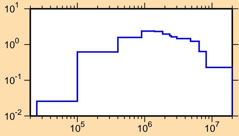
\sigma vs. E for ^{253}\text{Cf}(n,\text{inel.})
