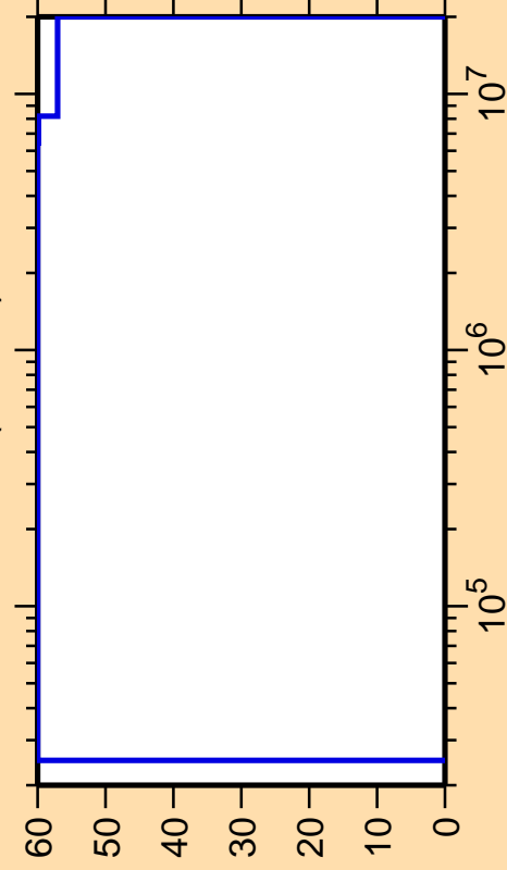
\Delta\sigma/\sigma vs. E for ^{253}\text{Cf}(n,\text{inel.})
