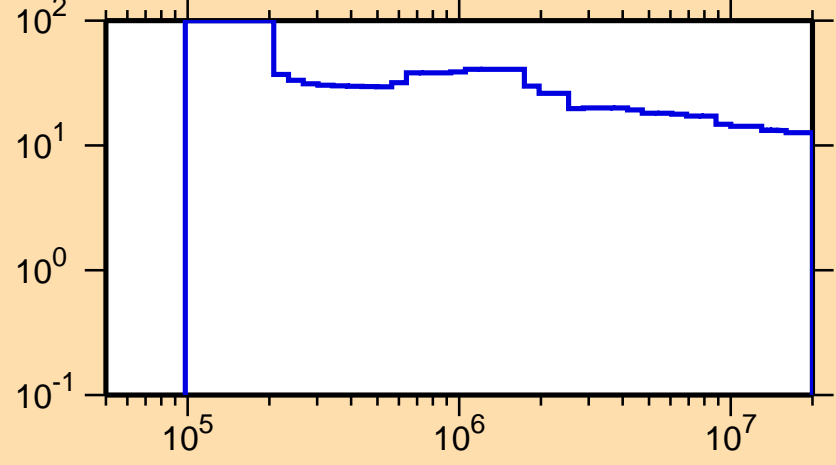
\Delta\sigma/\sigma vs. E for ^{254}\text{Cf}(n,\text{nonel.})
