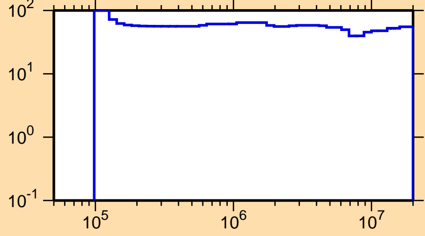
\Delta\sigma/\sigma vs. E for ^{254}\text{Cf}(n,\text{inel.})
