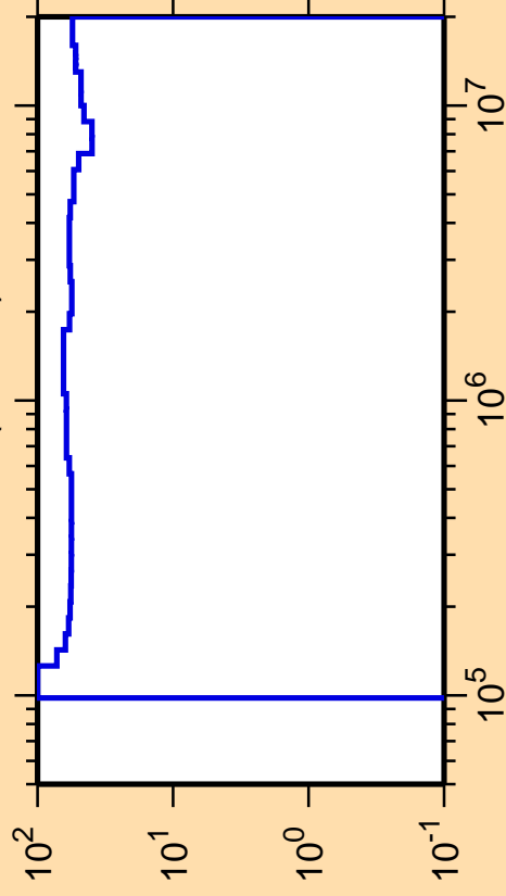
\Delta\sigma/\sigma vs. E for ^{254}\text{Cf}(n,\text{inel.})
