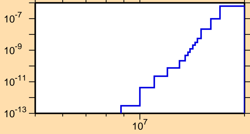
\sigma vs. E for ^{254}\text{Cf}(n,2n\alpha)
