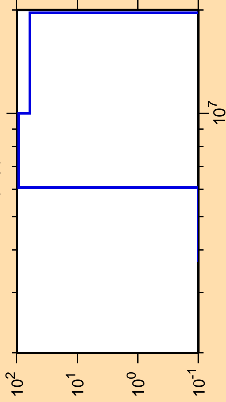
\Delta\sigma/\sigma vs. E for ^{254}\text{Cf}(n,p)
