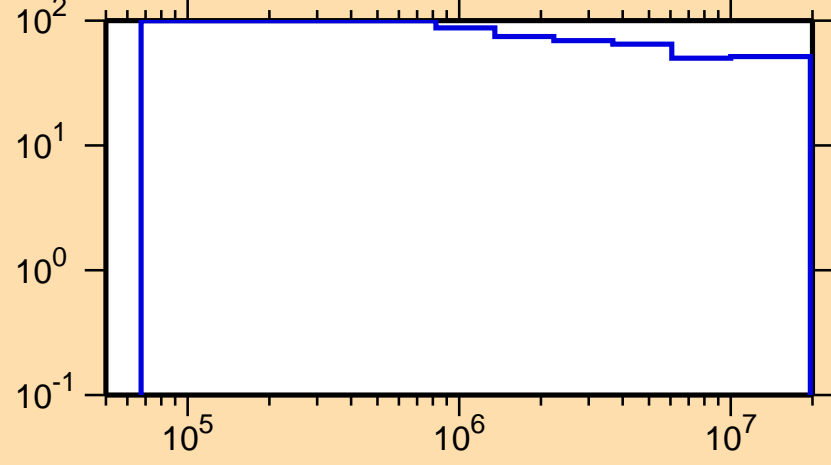
\Delta\sigma/\sigma vs. E for ^{254}\text{Cf}(n,ncont.)
