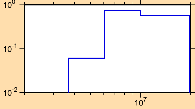
\sigma vs. E for ^{255}\text{Cf}(n,2n)
