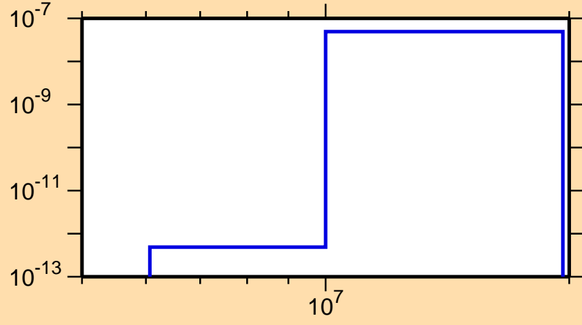
\sigma vs. E for ^{255}\text{Cf}(n,2n\alpha)
