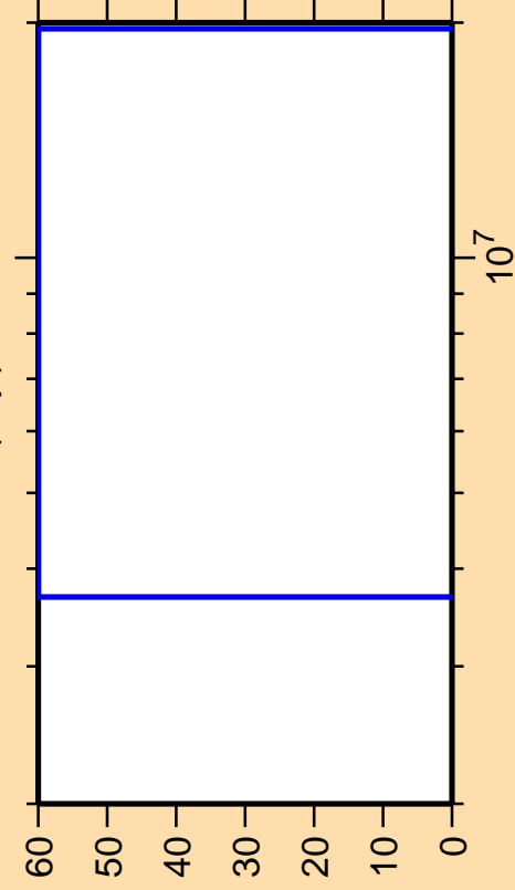
\Delta\sigma/\sigma vs. E for ^{255}\text{Cf}(n,p)
