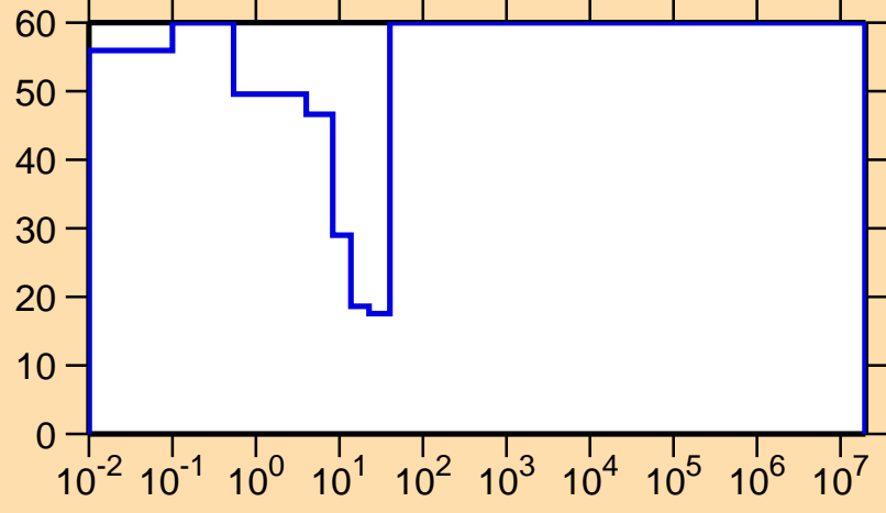
\Delta\sigma/\sigma vs. E for ^{255}\text{Cf}(n,\gamma)
