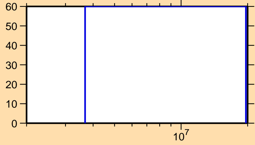
\Delta\sigma/\sigma vs. E for ^{255}\text{Cf}(n,ncont.)
