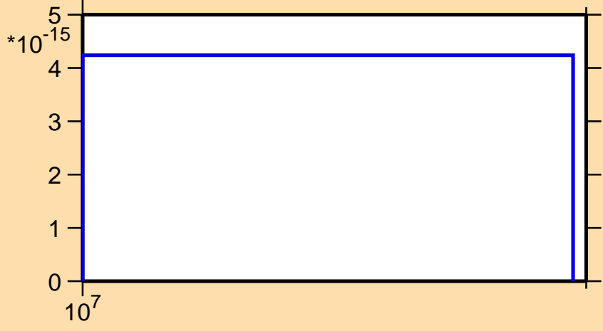
\sigma vs. E for ^{255}\text{Cf}(n,\text{He}3)
