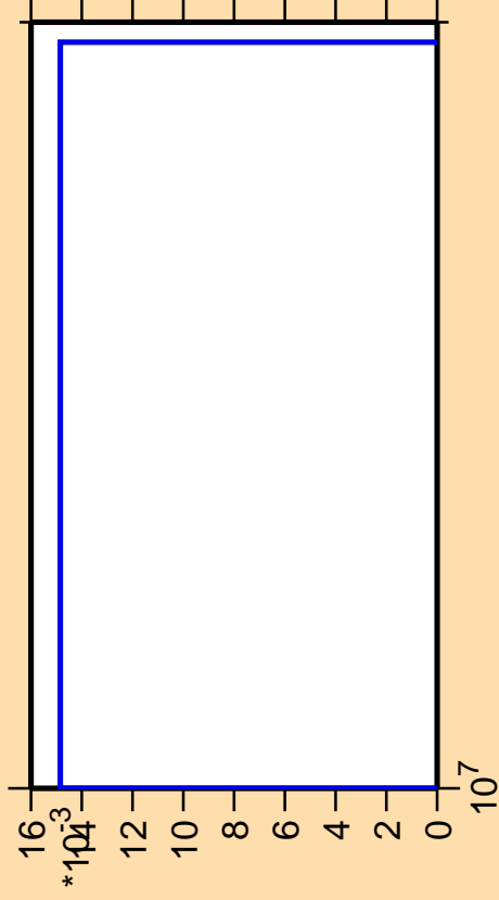
\Delta\sigma/\sigma vs. E for ^{255}\text{Cf}(n,\text{He}3)
