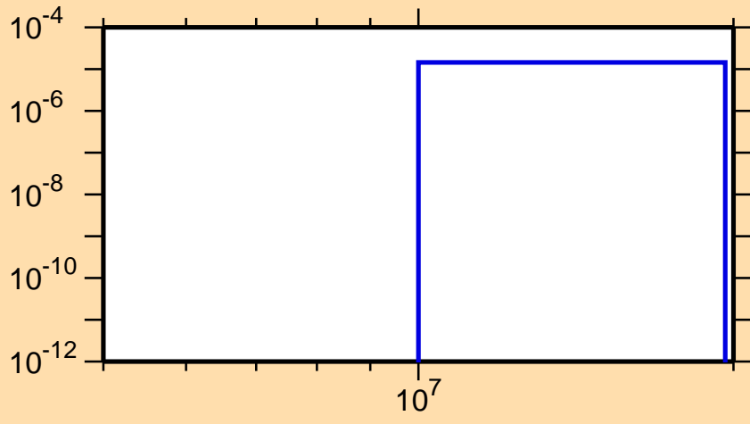
\sigma vs. E for ^{255}\text{Cf}(n,np)
