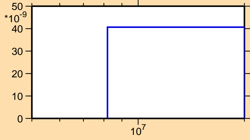
\sigma vs. E for ^{255}\text{Cf}(n,2n\alpha)
