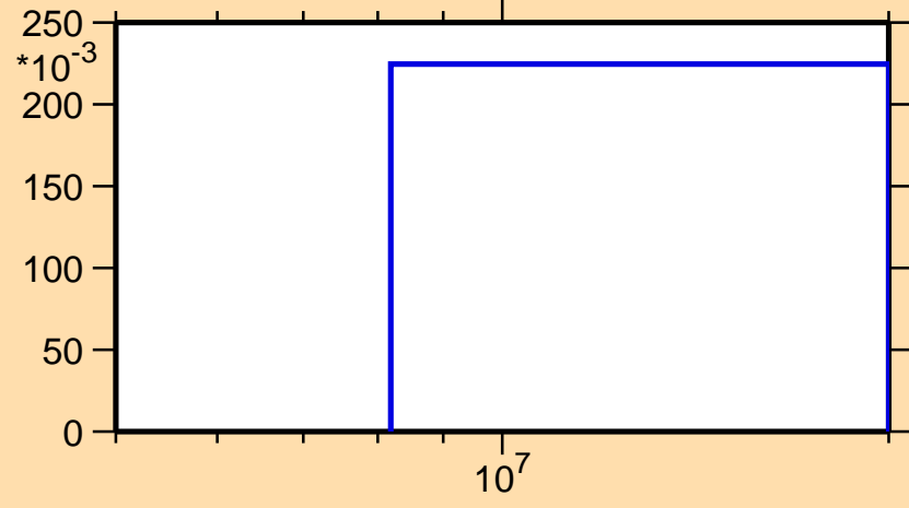
\sigma vs. E for ^{255}\text{Cf}(n,3n)
