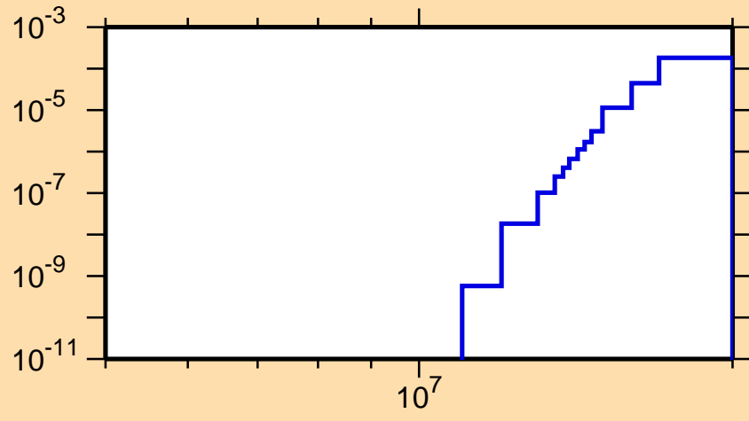
\sigma vs. E for ^{256}\text{Cf}(n,np)
