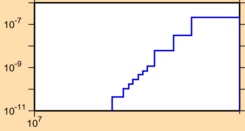
\sigma vs. E for ^{256}\text{Cf}(n,2n\alpha)
