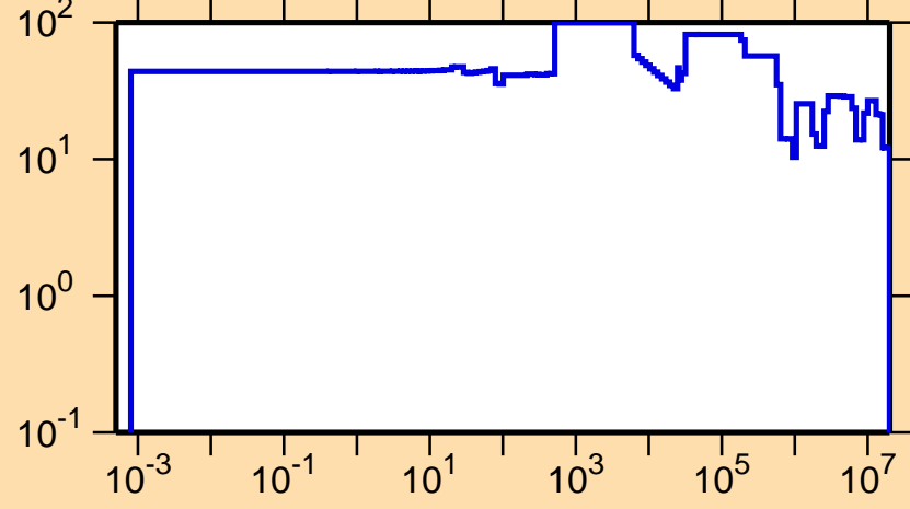
\Delta\sigma/\sigma vs. E for ^{256}\text{Cf}(n,\text{el.})
