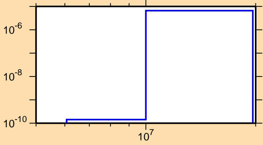
\sigma vs. E for ^{256}\text{Cf}(n,\alpha)
