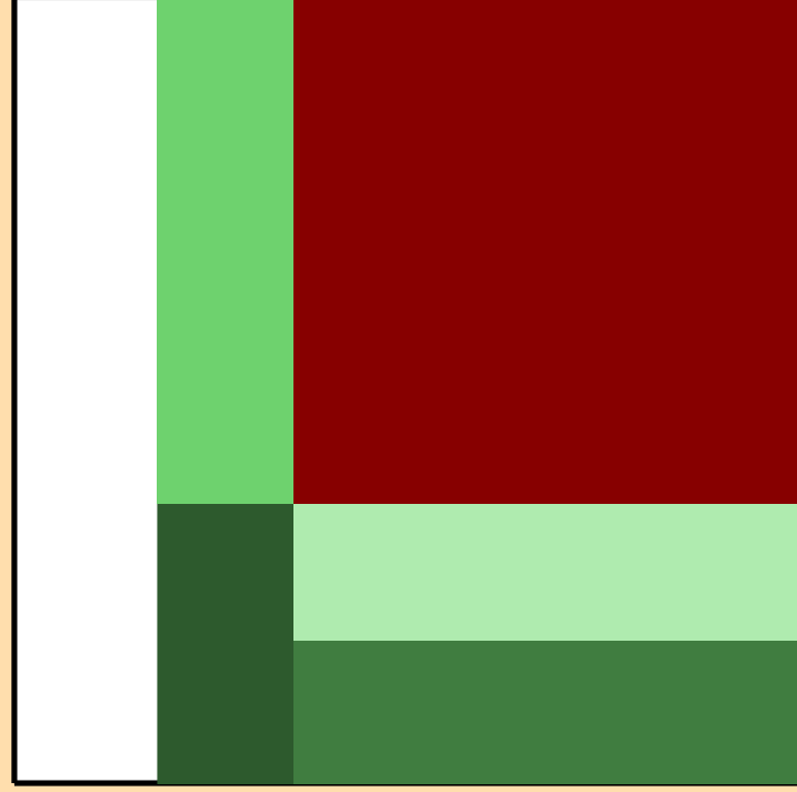
\Delta\sigma/\sigma vs. E for ^{256}\text{Cf}(n,p)
