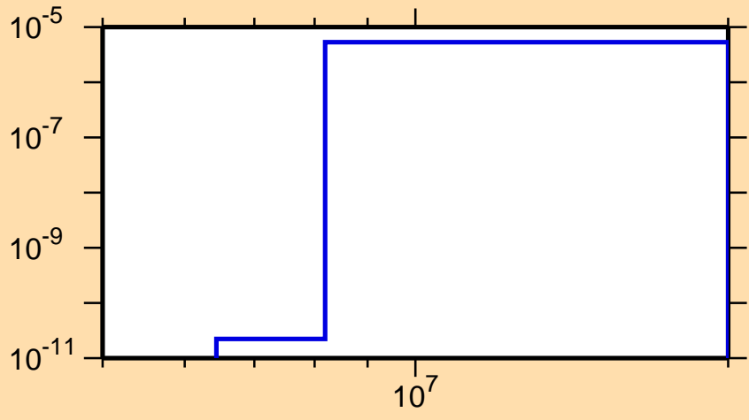
\sigma vs. E for ^{256}\text{Cf}(n,\alpha)
