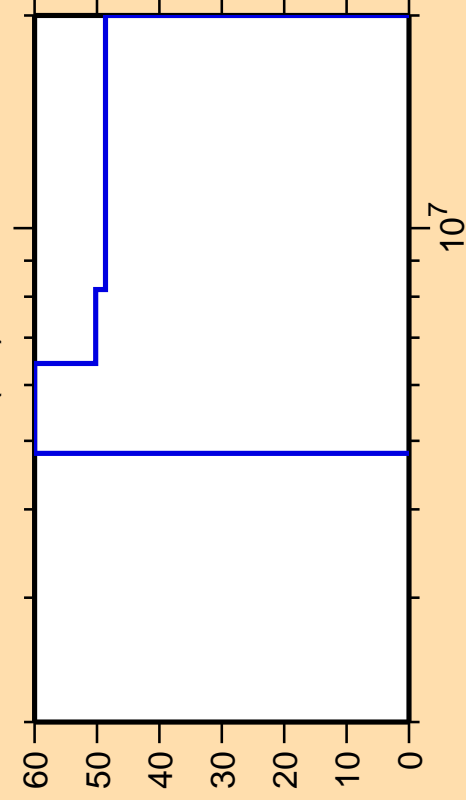
\Delta\sigma/\sigma vs. E for ^{256}\text{Cf}(n,f)
