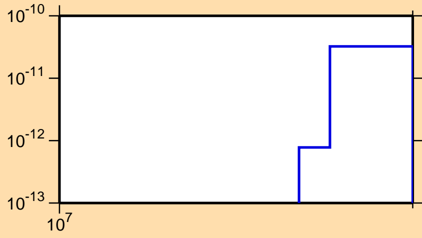
\sigma vs. E for ^{232}\text{Cm}(n,\text{nd})
