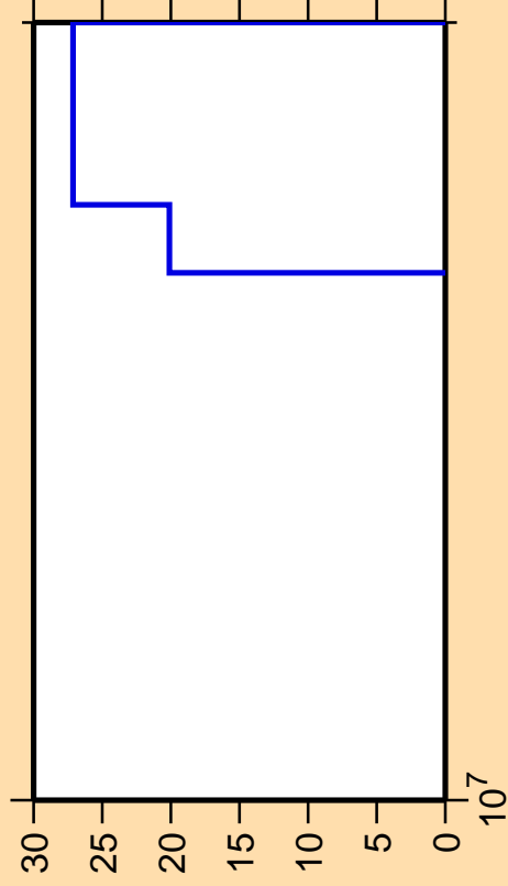
\Delta\sigma/\sigma vs. E for ^{232}\text{Cm} (mt117)
