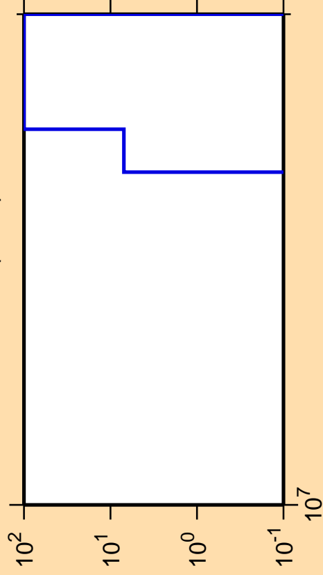
\Delta\sigma/\sigma vs. E for ^{232}\text{Cm}(n,\text{nd})
