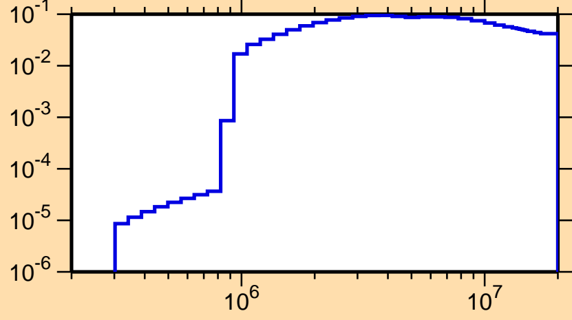
\sigma vs. E for ^{232}\text{Cm}(n,n\text{cont.})
