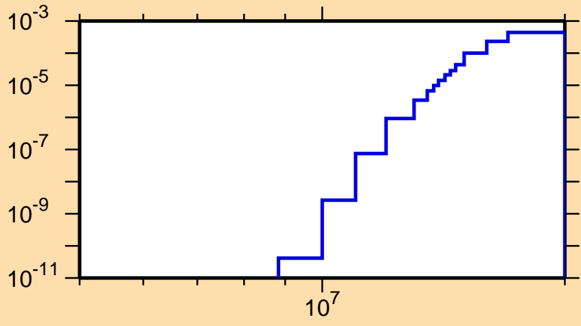
\sigma vs. E for ^{232}\text{Cm}(n,t)
