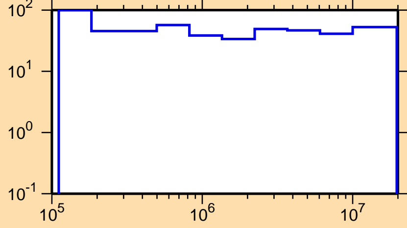
\Delta\sigma/\sigma vs. E for ^{232}\text{Cm}(n,\text{inel.})
