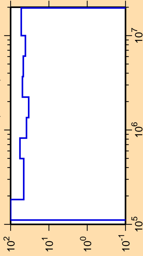
\Delta\sigma/\sigma vs. E for ^{232}\text{Cm}(n,\text{inel.})
