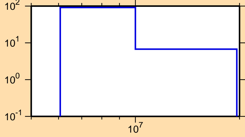
\Delta\sigma/\sigma vs. E for ^{232}\text{Cm}(n,2n)
