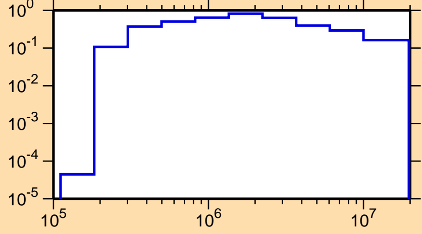
\sigma vs. E for ^{232}\text{Cm}(n,\text{inel.})
