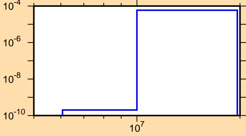
\sigma vs. E for ^{232}\text{Cm}(n,np)
