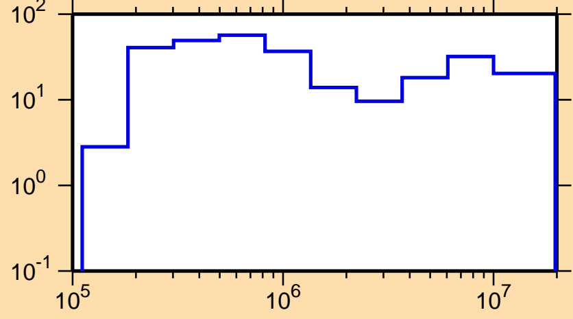
\Delta\sigma/\sigma vs. E for ^{232}\text{Cm}(n,\text{tot.})
