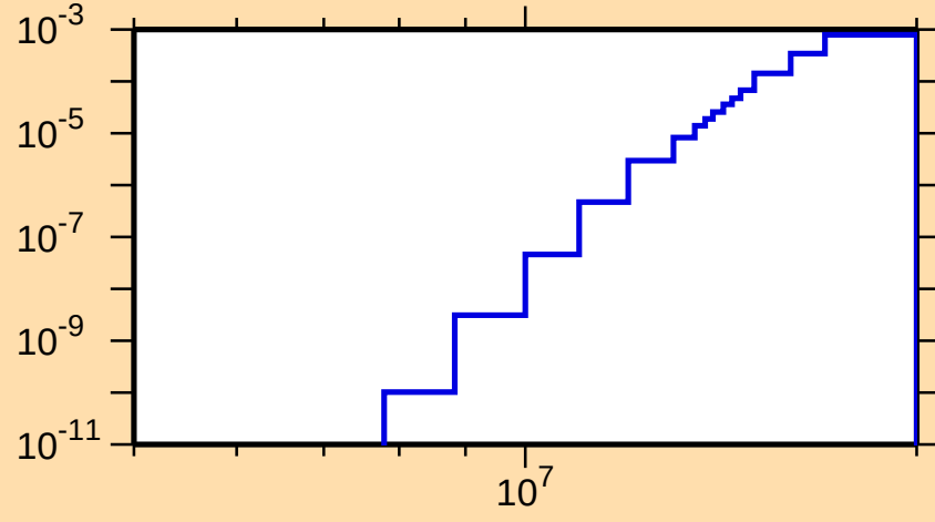
\sigma vs. E for ^{233}\text{Cm}(n,np)
