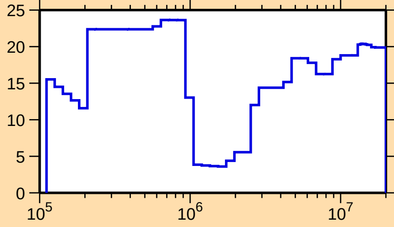
\Delta\sigma/\sigma vs. E for ^{233}\text{Cm}(n,n\text{oncl.})
