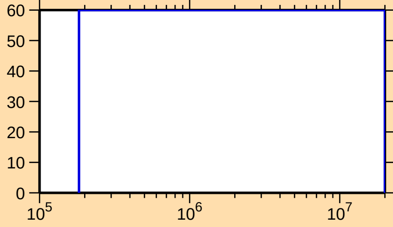
\Delta\sigma/\sigma vs. E for ^{233}\text{Cm}(n,n_1)
