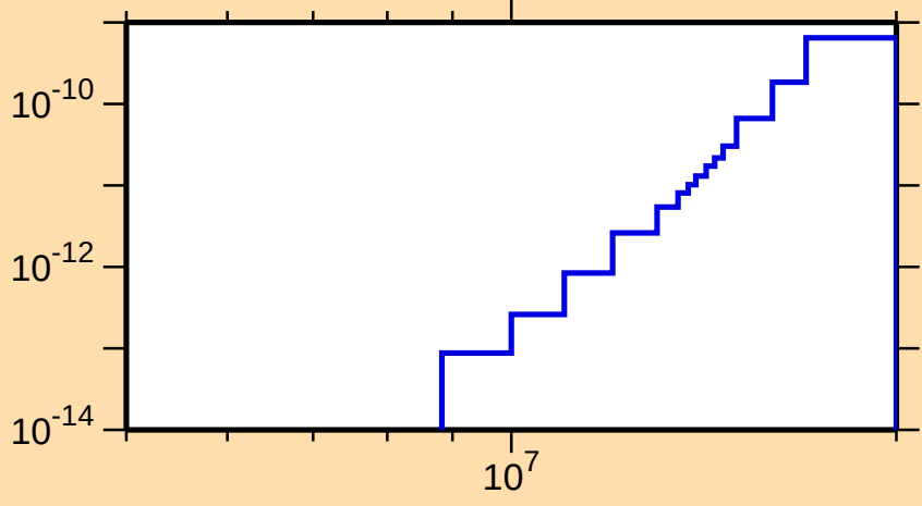
\sigma vs. E for ^{233}\text{Cm}(n,p\alpha)
