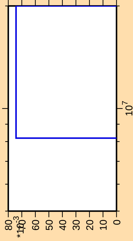
\Delta\sigma/\sigma vs. E for ^{233}\text{Cm}(n,nt)
