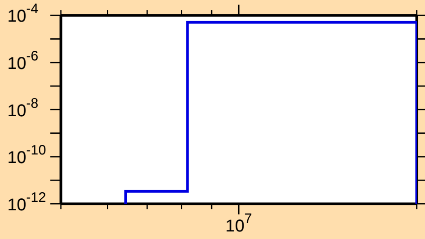
\sigma vs. E for ^{233}\text{Cm}(n,np)
