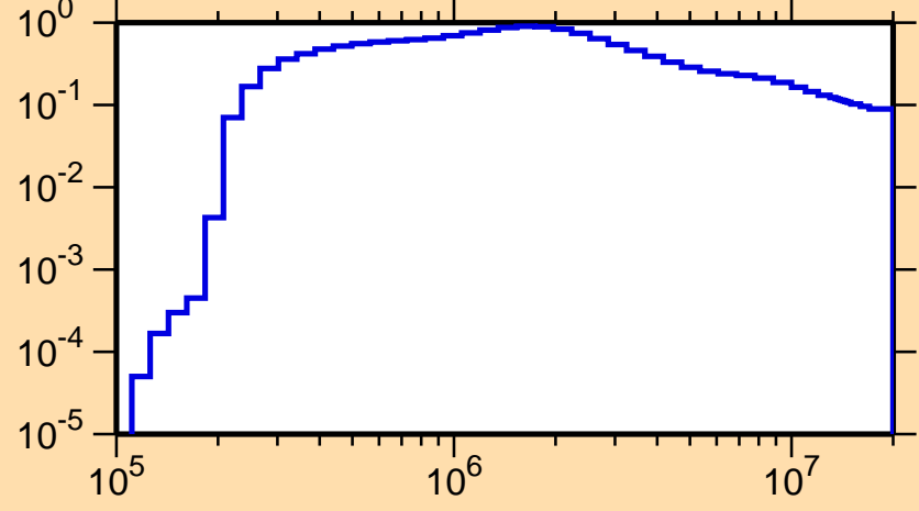
\sigma vs. E for ^{234}\text{Cm}(n,\text{inel.})
