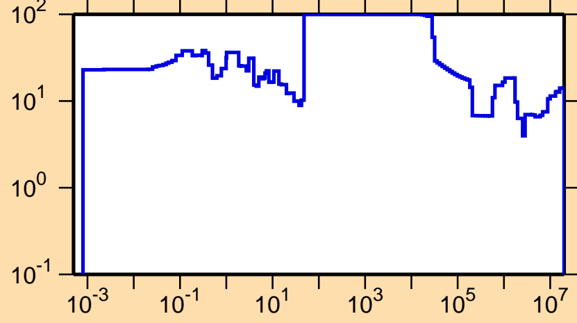
\Delta\sigma/\sigma vs. E for ^{234}\text{Cm}(n,f)
