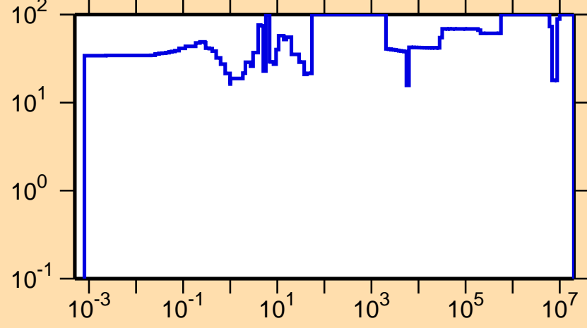
\Delta\sigma/\sigma vs. E for ^{234}\text{Cm}(n,\gamma)
