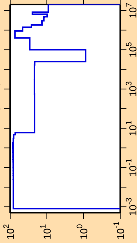
\Delta\sigma/\sigma vs. E for ^{235}\text{Cm}(n,\text{el.})
