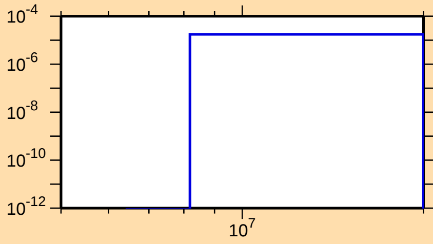
\sigma vs. E for ^{235}\text{Cm}(n,np)
