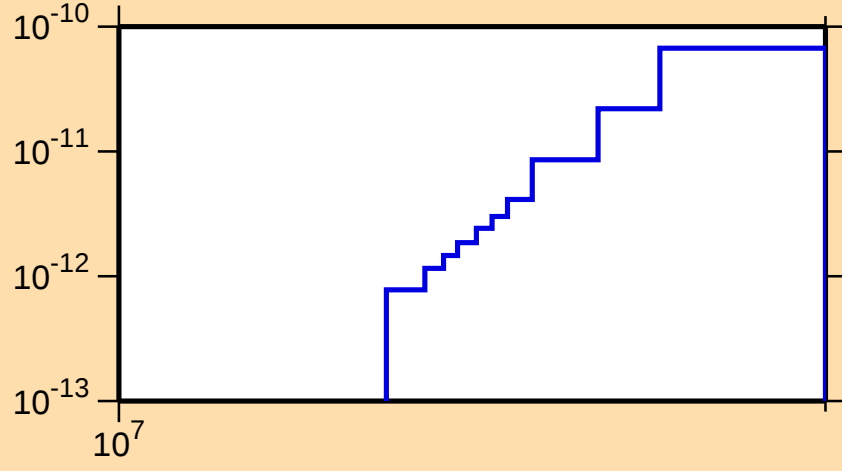
\sigma vs. E for ^{236}\text{Cm}(n,p\alpha)
