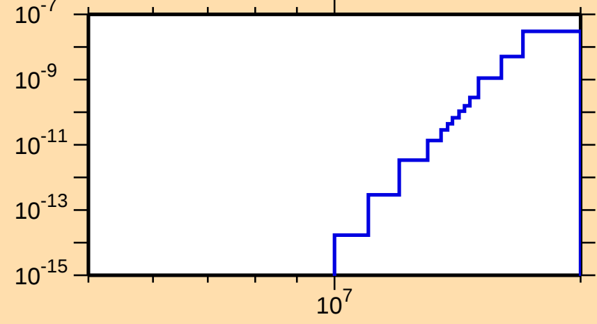
\sigma vs. E for ^{236}\text{Cm}(n,\text{He3})
