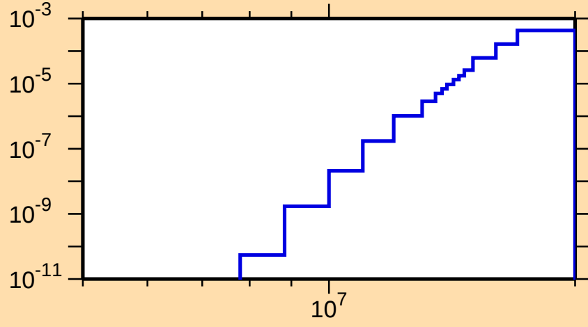
\sigma vs. E for ^{236}\text{Cm}(n,np)
