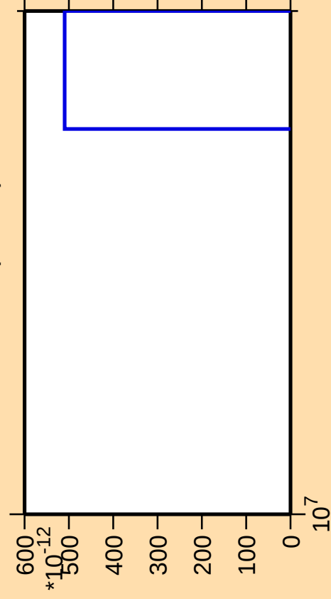
\Delta\sigma/\sigma vs. E for ^{236}\text{Cm}(\text{mt } 42)
