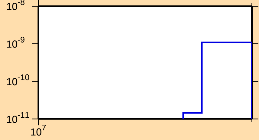
\sigma vs. E for ^{236}\text{Cm}(n,2np)
