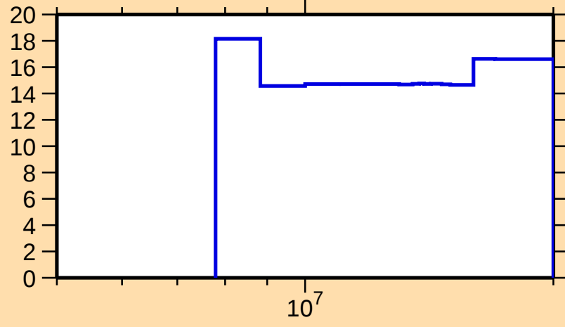
\Delta\sigma/\sigma vs. E for ^{236}\text{Cm}(n,\text{el.})
