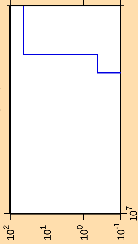
\Delta\sigma/\sigma vs. E for ^{236}\text{Cm}(n,nt)
