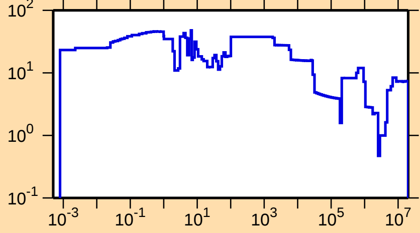
\Delta\sigma/\sigma vs. E for ^{236}\text{Cm}(n,\text{tot.})
