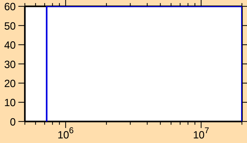
\Delta\sigma/\sigma vs. E for ^{236}\text{Cm}(n,n\text{cont.})
