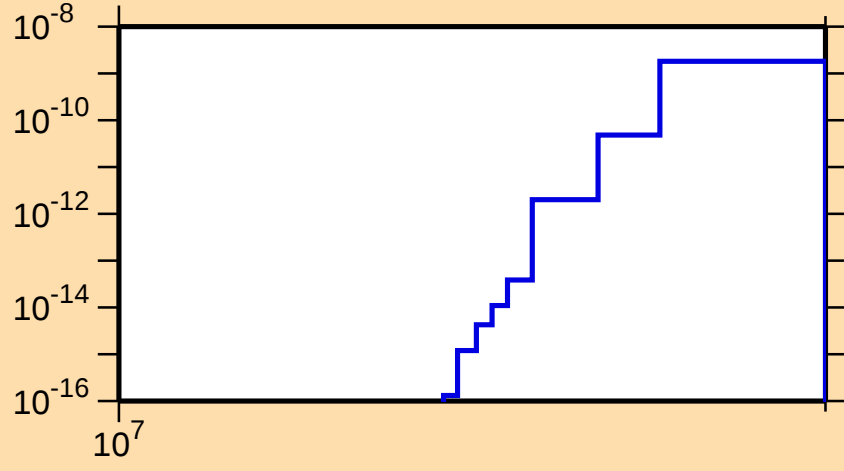
\sigma vs. E for ^{236}\text{Cm}(n,\text{nd})
