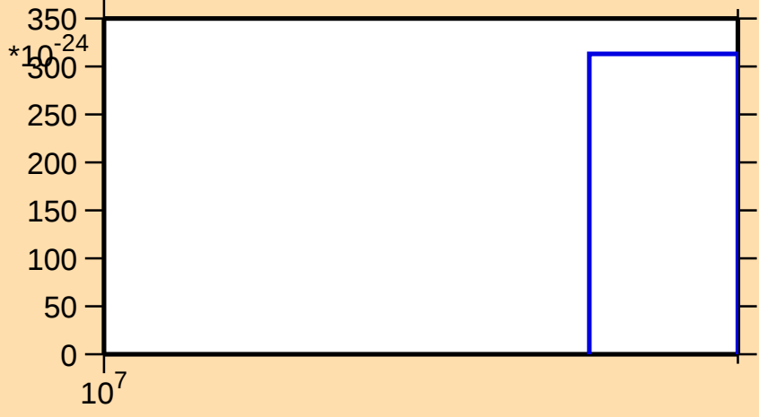
\sigma vs. E for ^{236}\text{Cm}(\text{mt } 42)
