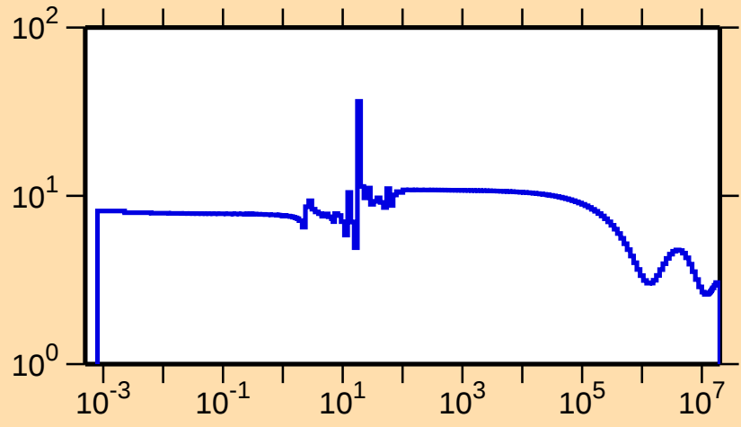
\sigma vs. E for ^{236}\text{Cm}(n,\text{el.})
