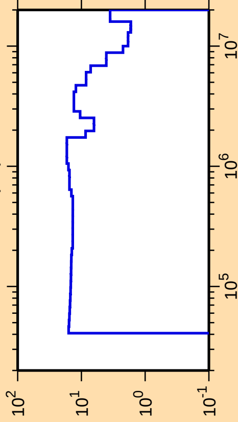
\Delta\sigma/\sigma vs. E for ^{236}\text{Cm}(n,f)
