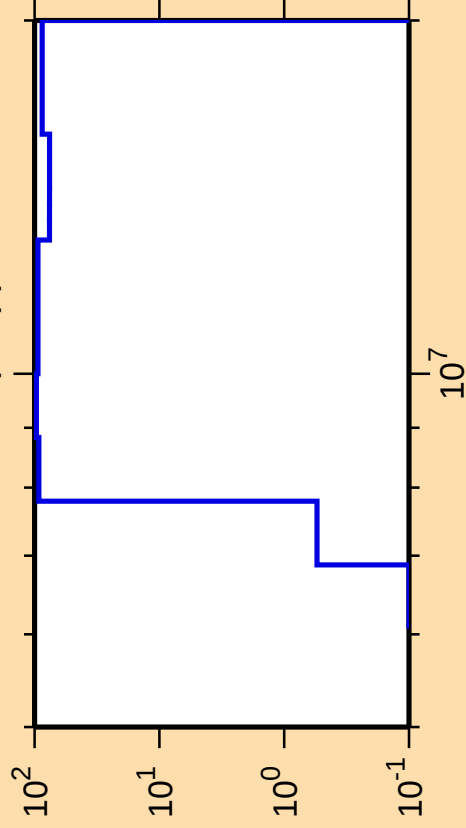
\Delta\sigma/\sigma vs. E for ^{236}\text{Cm}(n,np)
