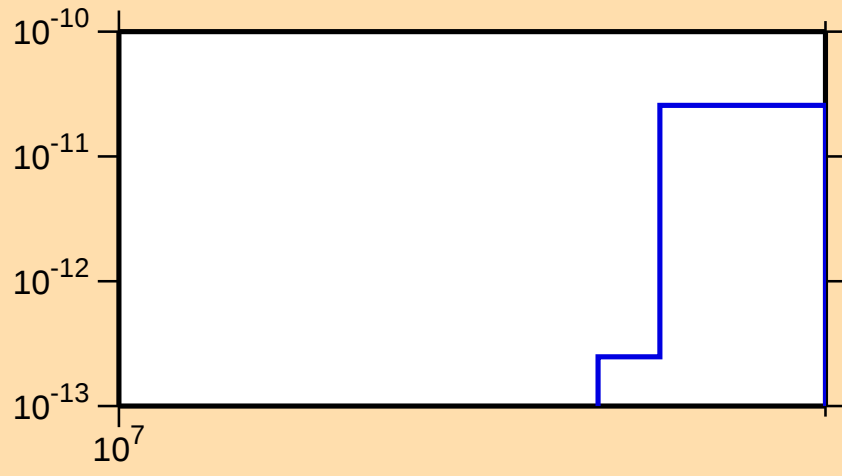
\sigma vs. E for ^{236}\text{Cm}(n,nt)
