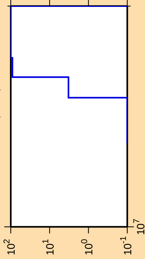
\Delta\sigma/\sigma vs. E for ^{236}\text{Cm}(n,\text{nd})
