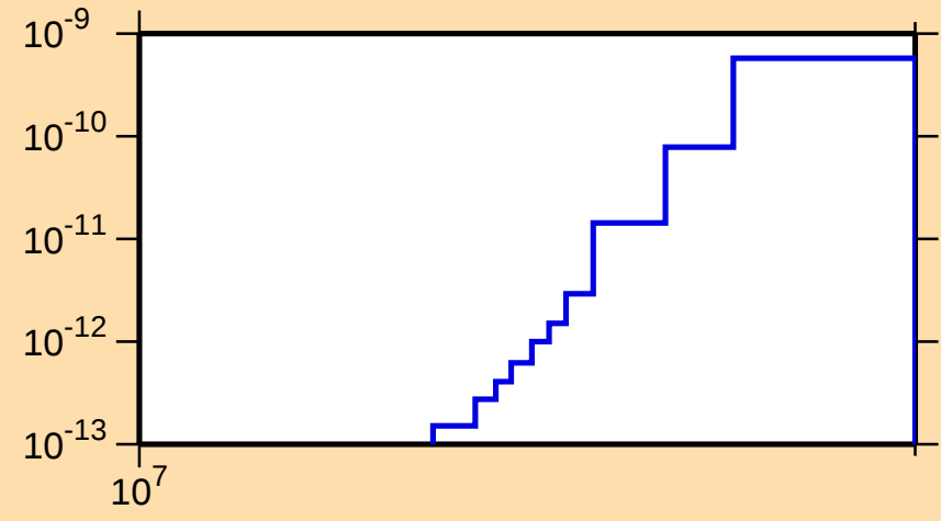
\sigma vs. E for ^{236}\text{Cm}(n,2n\alpha)
