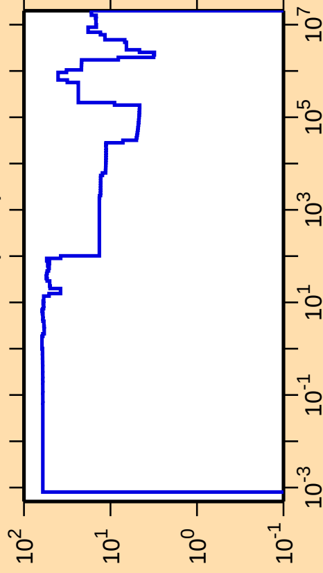
\Delta\sigma/\sigma vs. E for ^{236}\text{Cm}(n,\text{el.})
