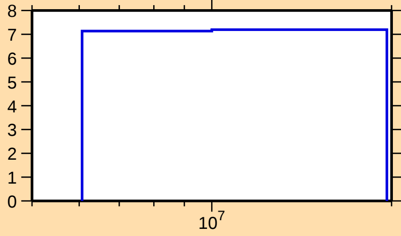
\Delta\sigma/\sigma vs. E for ^{236}\text{Cm}(n,\text{tot.})
