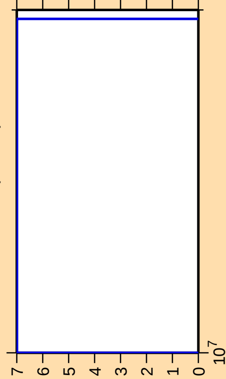
\Delta\sigma/\sigma vs. E for ^{236}\text{Cm}(n,2n\alpha)
