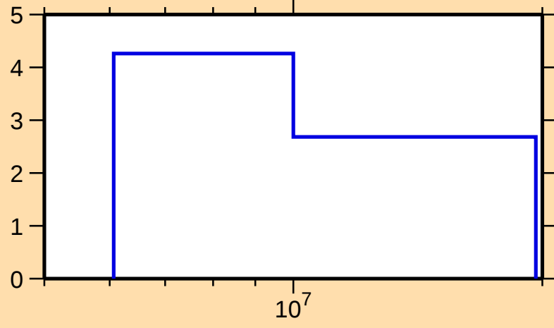
\Delta\sigma/\sigma vs. E for ^{236}\text{Cm}(n,\text{nonel.})
