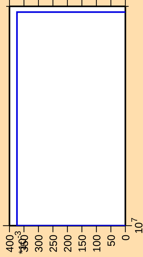
\Delta\sigma/\sigma vs. E for ^{236}\text{Cm}(n,nt)
