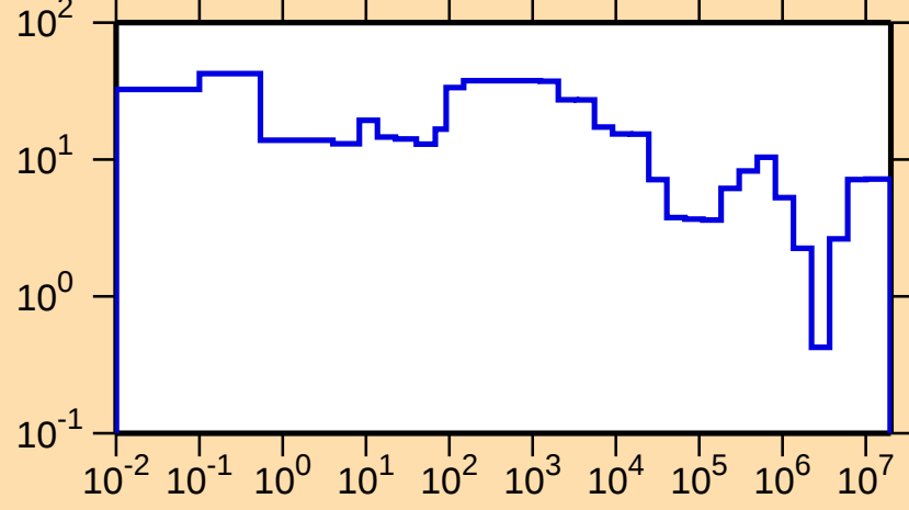
\Delta\sigma/\sigma vs. E for ^{236}\text{Cm}(n,\text{tot.})
