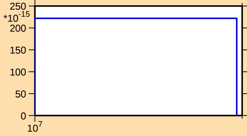
\sigma vs. E for ^{236}\text{Cm}(n,nt)
