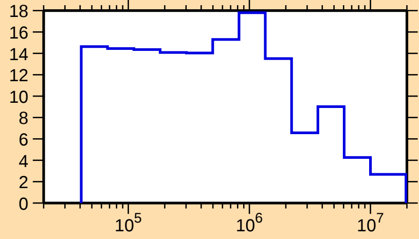
\Delta\sigma/\sigma vs. E for ^{236}\text{Cm}(n,\text{nonel.})
