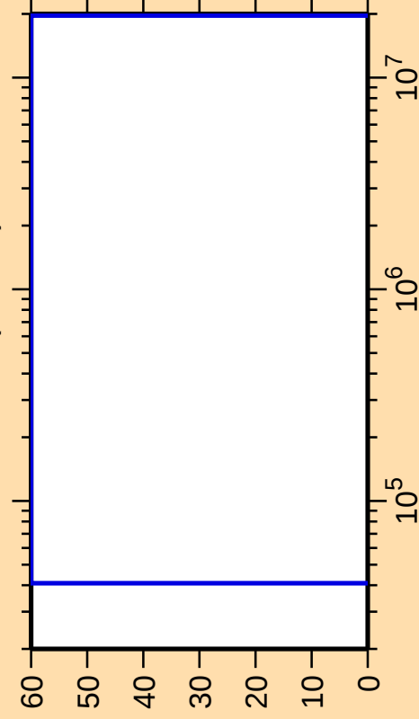
\Delta\sigma/\sigma vs. E for ^{236}\text{Cm}(n,\text{inel.})
