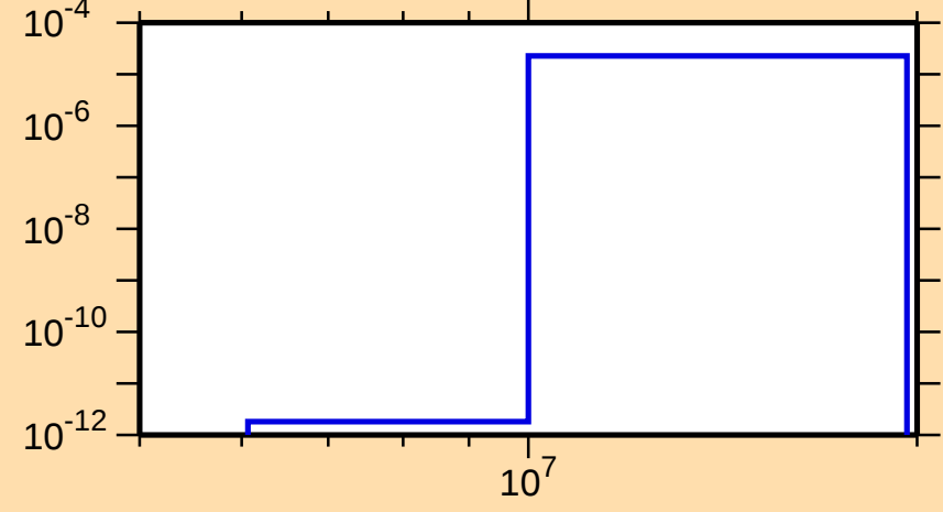
\sigma vs. E for ^{236}\text{Cm}(n,t)
