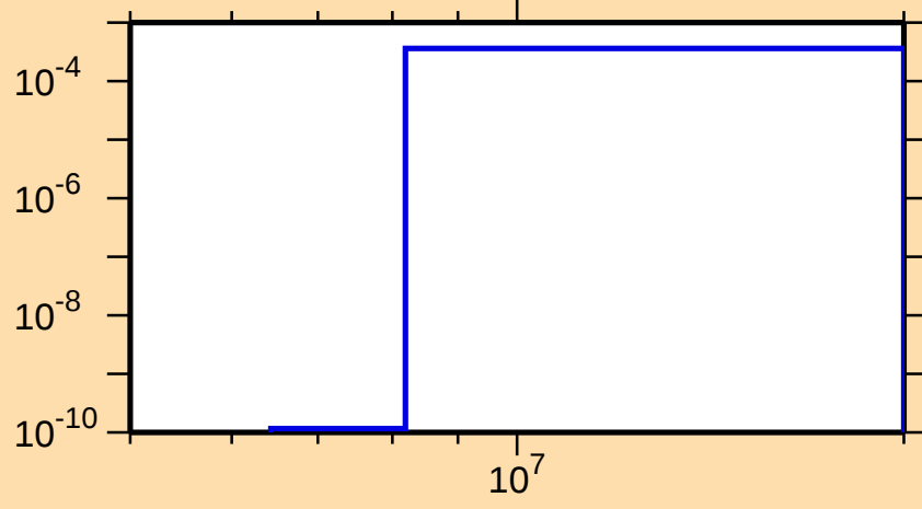
\sigma vs. E for ^{236}\text{Cm}(n,d)
