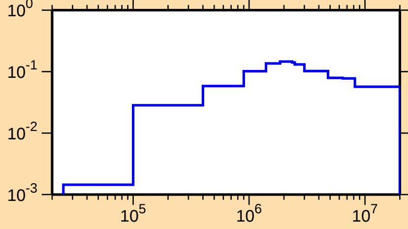
\sigma vs. E for ^{236}\text{Cm}(n,\text{inel.})
