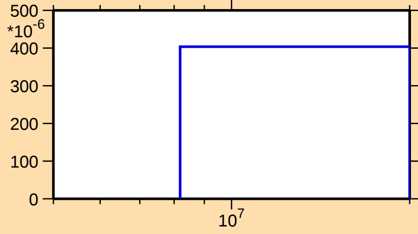
\sigma vs. E for ^{236}\text{Cm}(n,2n)
