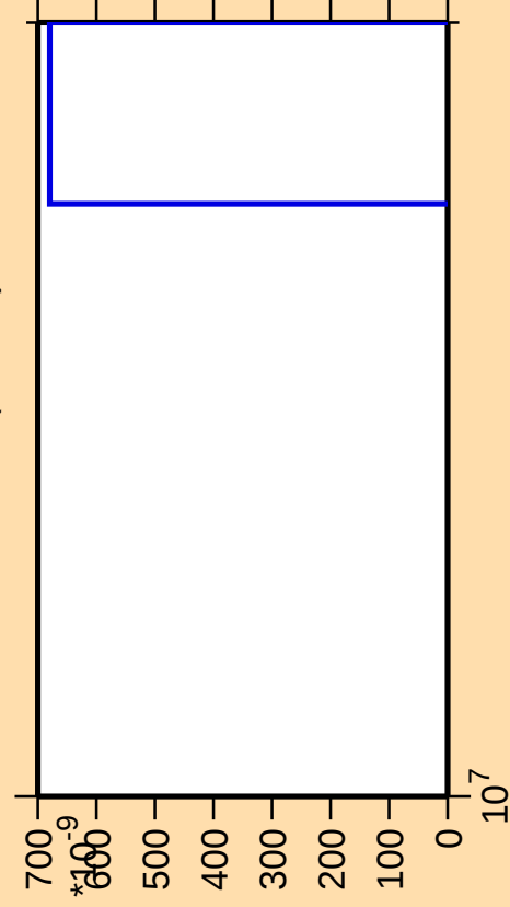
\Delta\sigma/\sigma vs. E for ^{237}\text{Cm}(\text{mt } 42)
