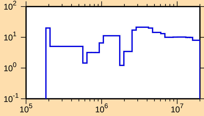
\Delta\sigma/\sigma vs. E for ^{237}\text{Cm}(n,f)
