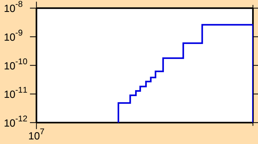
\sigma vs. E for ^{237}\text{Cm}(n,2n\alpha)
