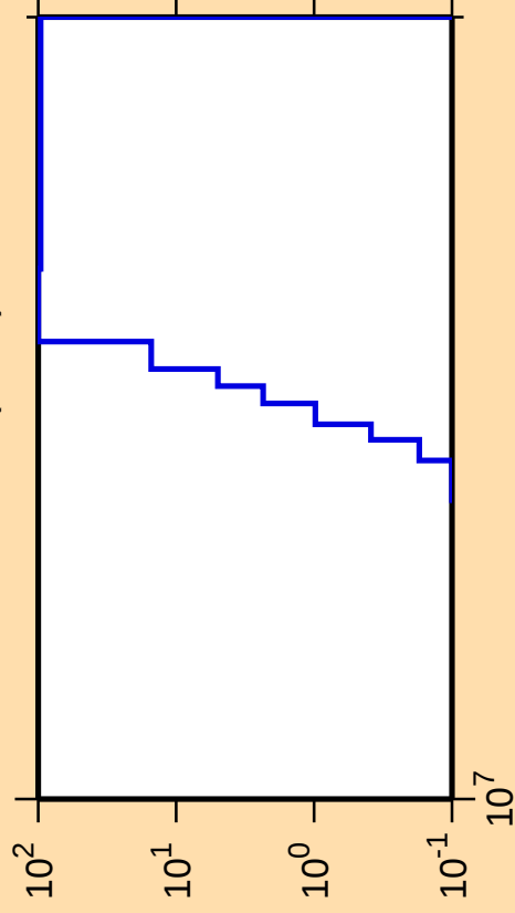
\Delta\sigma/\sigma vs. E for ^{237}\text{Cm}(n,\text{nd})
