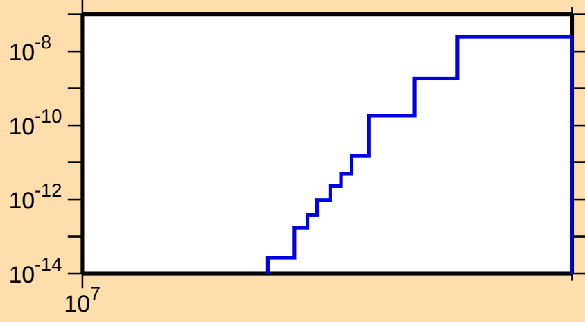
\sigma vs. E for ^{237}\text{Cm}(n,\text{nd})
