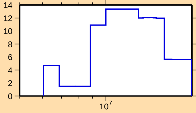
\Delta\sigma/\sigma vs. E for ^{237}\text{Cm}(n,\text{tot.})
