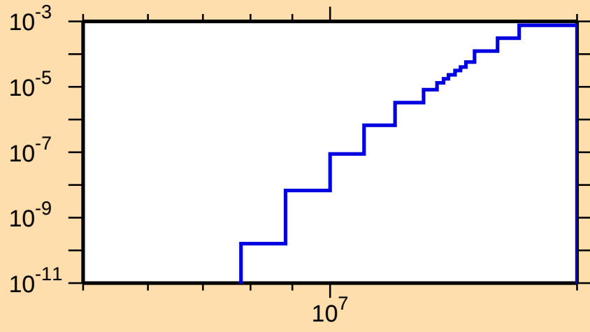
\sigma vs. E for ^{237}\text{Cm}(n,np)
