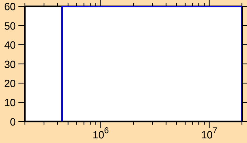
\Delta\sigma/\sigma vs. E for ^{237}\text{Cm}(n,n\text{cont.})
