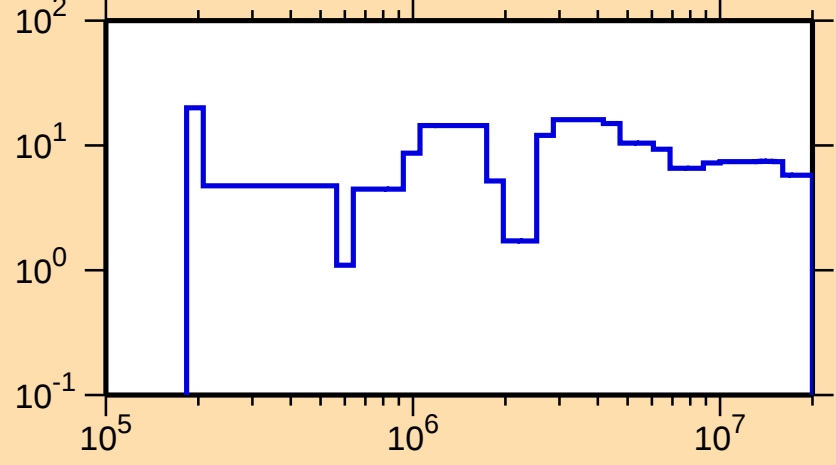
\Delta\sigma/\sigma vs. E for ^{237}\text{Cm}(n,\text{nonel.})
