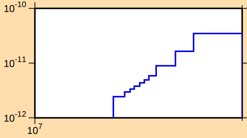
\sigma vs. E for ^{237}\text{Cm}(n,p\alpha)
