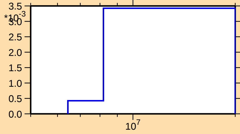
\sigma vs. E for ^{237}\text{Cm}(n,2n)
