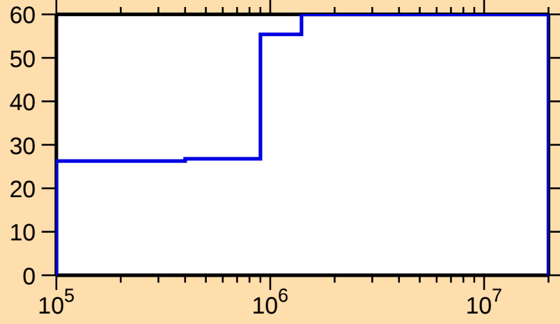
\Delta\sigma/\sigma vs. E for ^{237}\text{Cm}(n,n_1)
