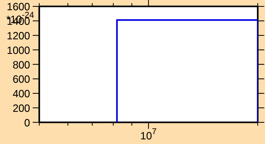
\sigma vs. E for ^{237}\text{Cm}(\text{mt } 42)
