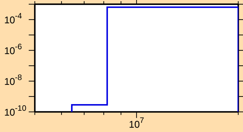
\sigma vs. E for ^{237}\text{Cm}(n,d)
