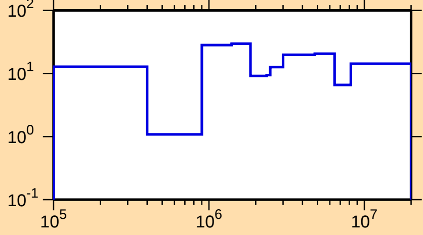
\Delta\sigma/\sigma vs. E for ^{237}\text{Cm}(n,\text{el.})
